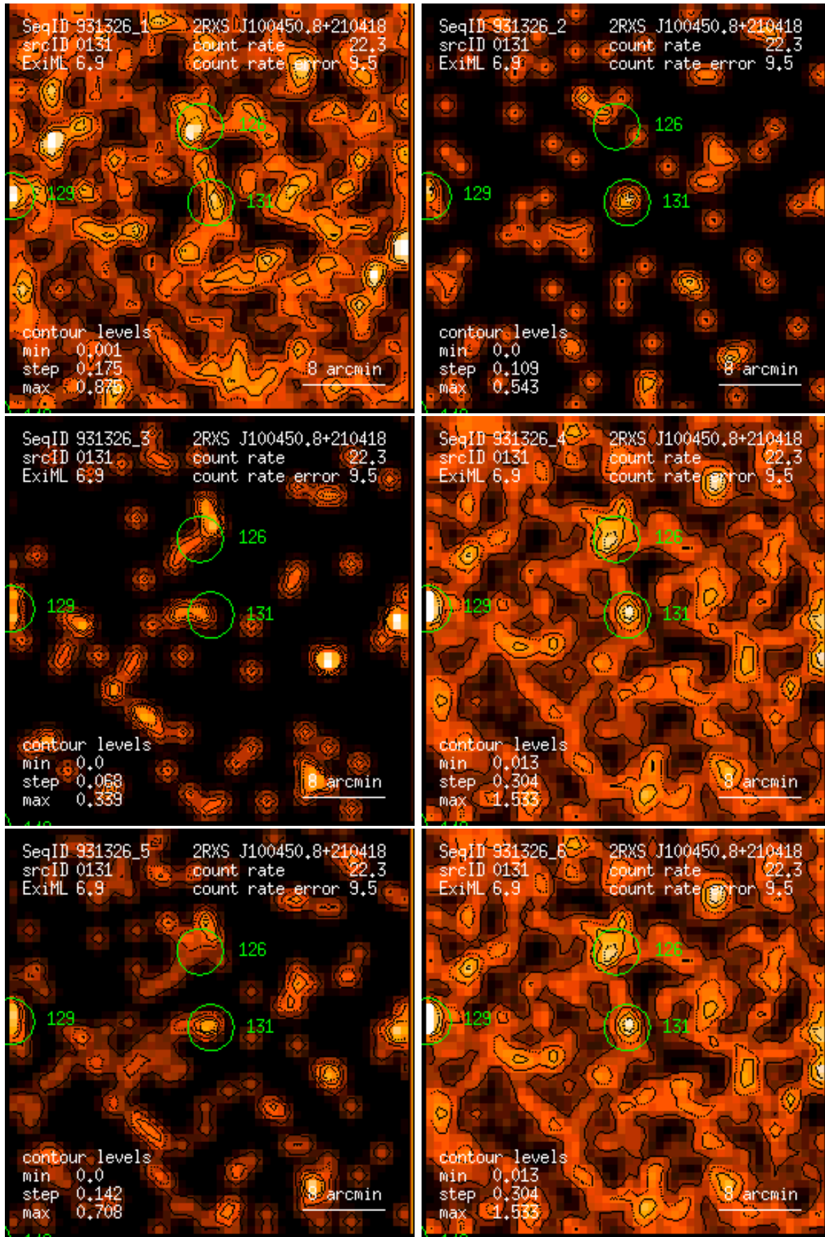
Figure 131: RASS 931326: detection 0131: band rate images, Gaussian filter: (1) PSPC channels 11 – 41, (2) 52 – 90, (3) 91 – 201, (4) 11 – 235, (5) 52 – 201, (6) 11 – 201. Broad band rates in counts/ks. Band rate contour levels in counts/ks/arcmin 2 .
