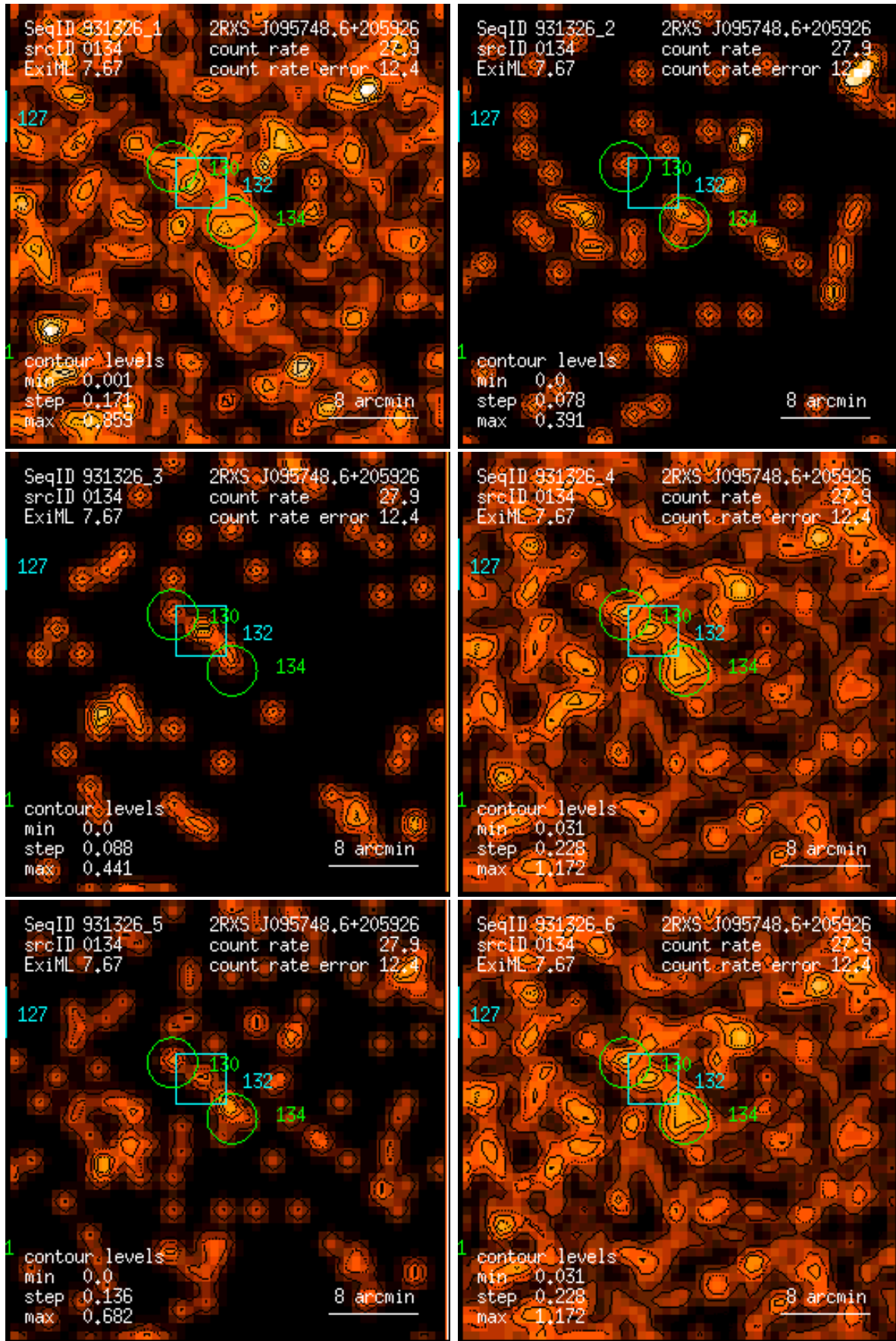
Figure 134: RASS 931326: detection 0134: band rate images, Gaussian filter: (1) PSPC channels 11 – 41, (2) 52 – 90, (3) 91 – 201, (4) 11 – 235, (5) 52 – 201, (6) 11 – 201. Broad band rates in counts/ks. Band rate contour levels in counts/ks/arcmin 2 .
