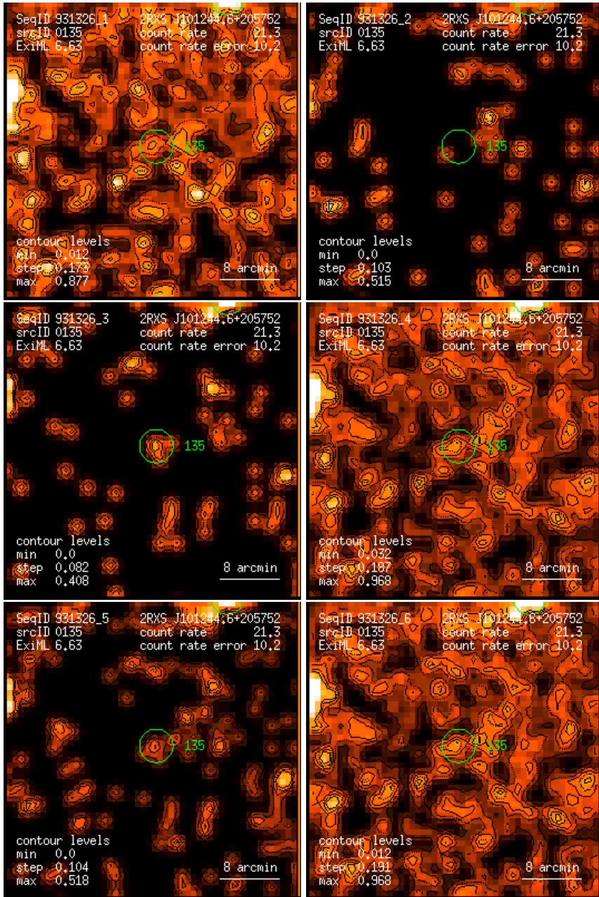
Figure 135: RASS 931326: detection 0135: band rate images, Gaussian filter: (1) PSPC channels 11 – 41, (2) 52 – 90, (3) 91 – 201, (4) 11 – 235, (5) 52 – 201, (6) 11 – 201. Broad band rates in counts/ks. Band rate contour levels in counts/ks/arcmin 2 .
