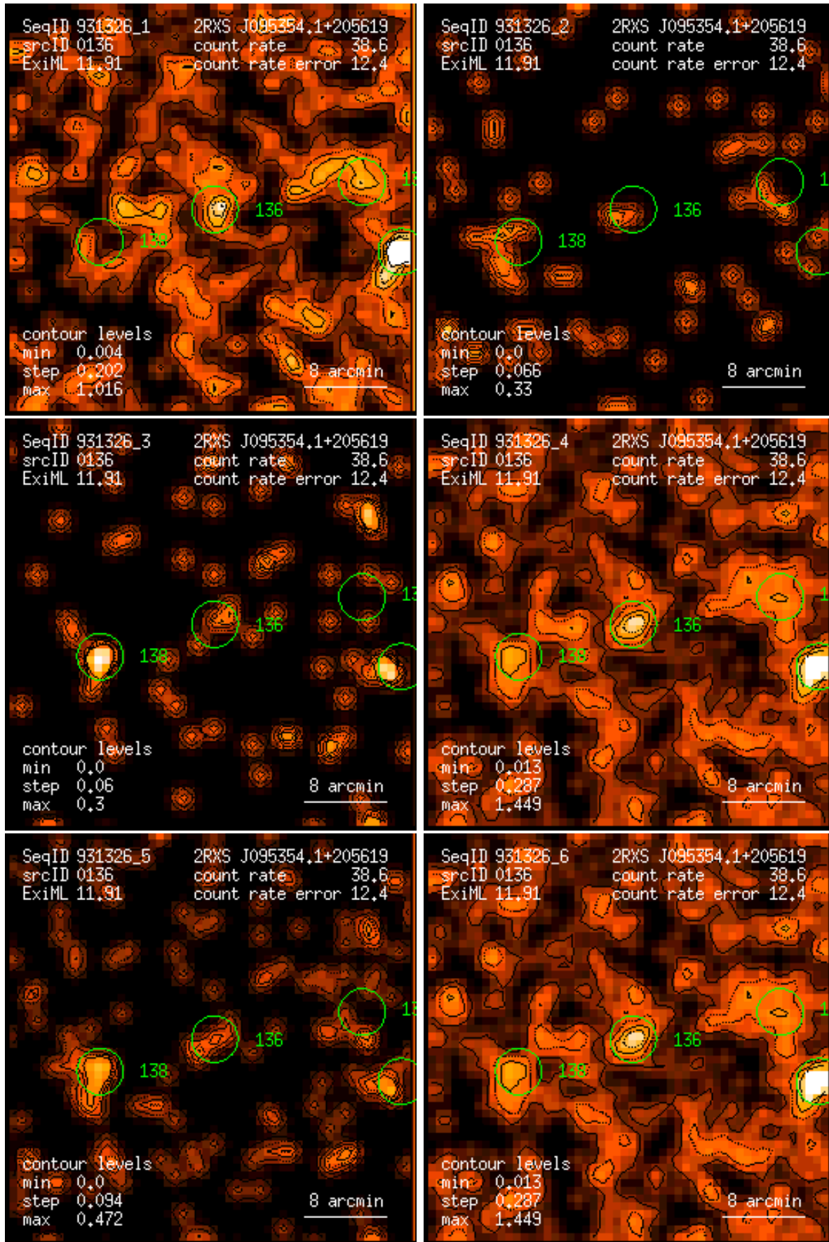
Figure 136: RASS 931326: detection 0136: band rate images, Gaussian filter: (1) PSPC channels 11 – 41, (2) 52 – 90, (3) 91 – 201, (4) 11 – 235, (5) 52 – 201, (6) 11 – 201. Broad band rates in counts/ks. Band rate contour levels in counts/ks/arcmin 2 .
