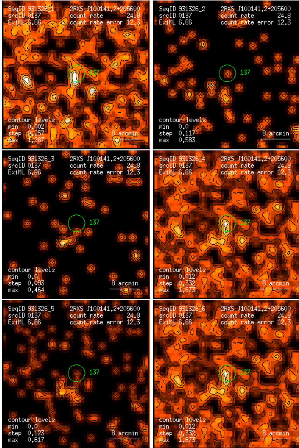
Figure 137: RASS 931326: detection 0137: band rate images, Gaussian filter: (1) PSPC channels 11 – 41, (2) 52 – 90, (3) 91 – 201, (4) 11 – 235, (5) 52 – 201, (6) 11 – 201. Broad band rates in counts/ks. Band rate contour levels in counts/ks/arcmin 2 .
