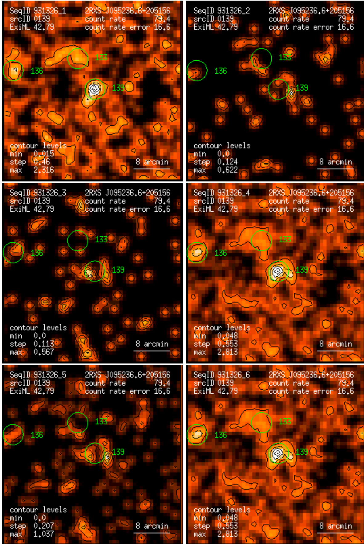
Figure 139: RASS 931326: detection 0139: band rate images, Gaussian filter: (1) PSPC channels 11 – 41, (2) 52 – 90, (3) 91 – 201, (4) 11 – 235, (5) 52 – 201, (6) 11 – 201. Broad band rates in counts/ks. Band rate contour levels in counts/ks/arcmin 2 .
