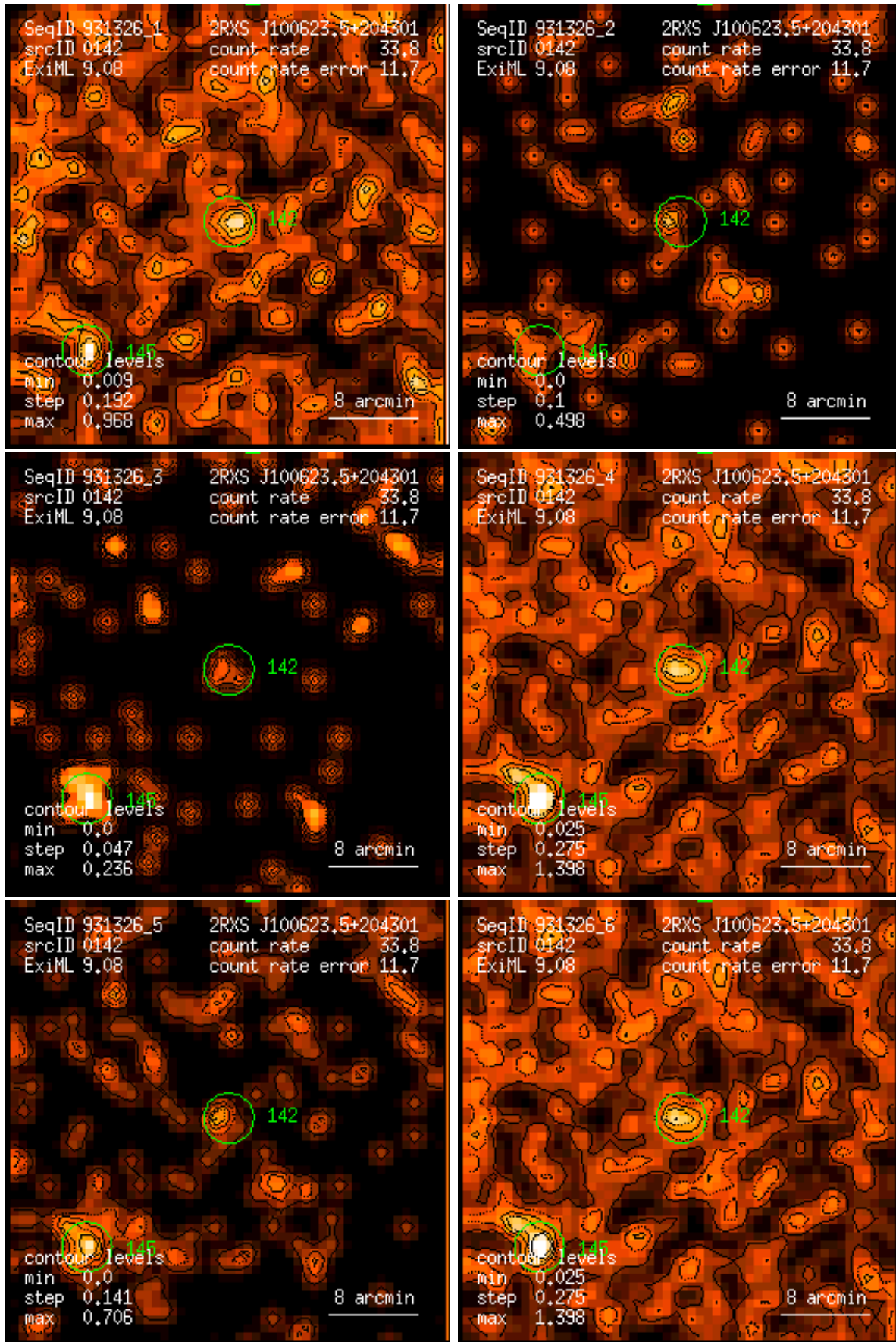
Figure 142: RASS 931326: detection 0142: band rate images, Gaussian filter: (1) PSPC channels 11 – 41, (2) 52 – 90, (3) 91 – 201, (4) 11 – 235, (5) 52 – 201, (6) 11 – 201. Broad band rates in counts/ks. Band rate contour levels in counts/ks/arcmin 2 .
