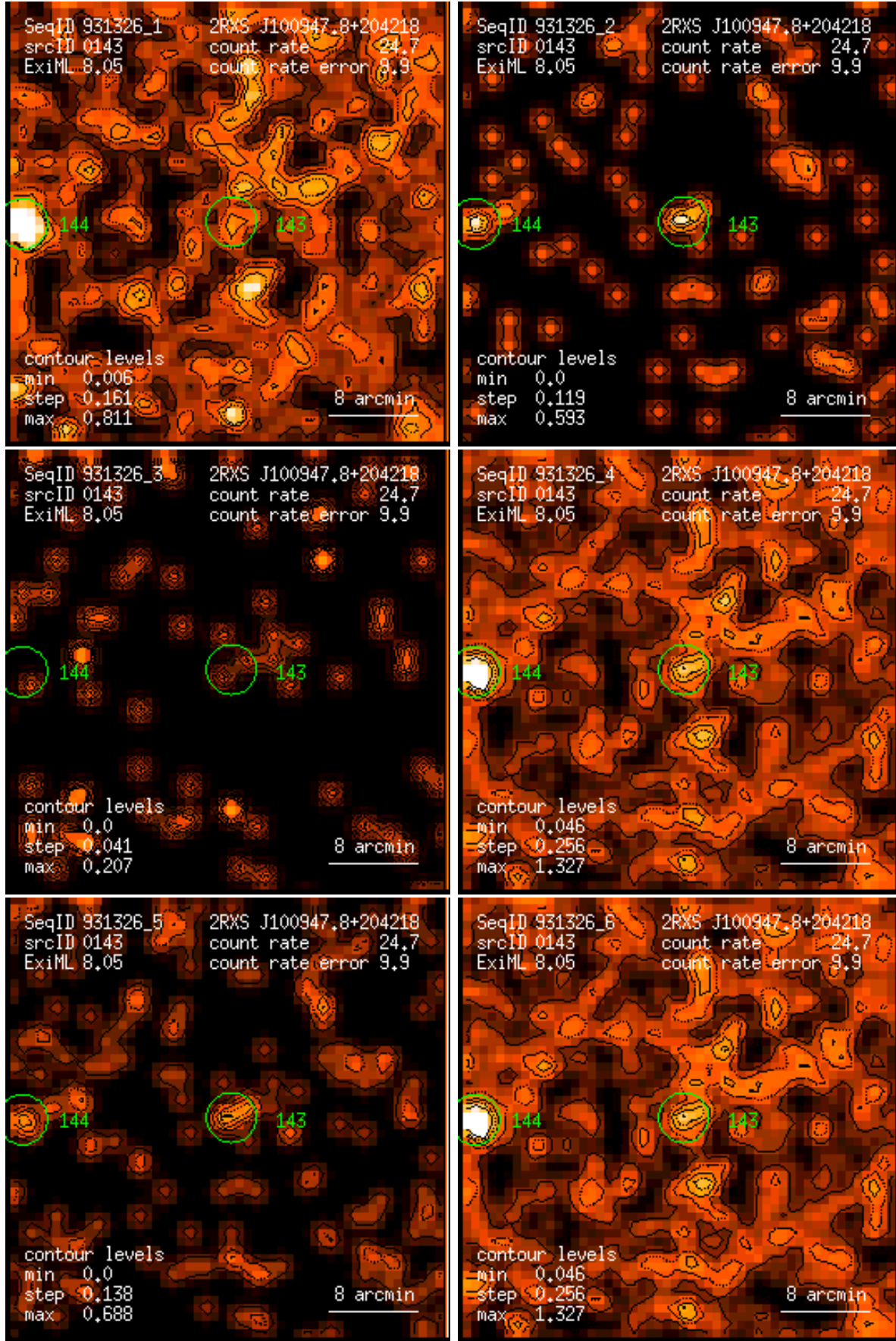
Figure 143: RASS 931326: detection 0143: band rate images, Gaussian filter: (1) PSPC channels 11 – 41, (2) 52 – 90, (3) 91 – 201, (4) 11 – 235, (5) 52 – 201, (6) 11 – 201. Broad band rates in counts/ks. Band rate contour levels in counts/ks/arcmin 2 .
