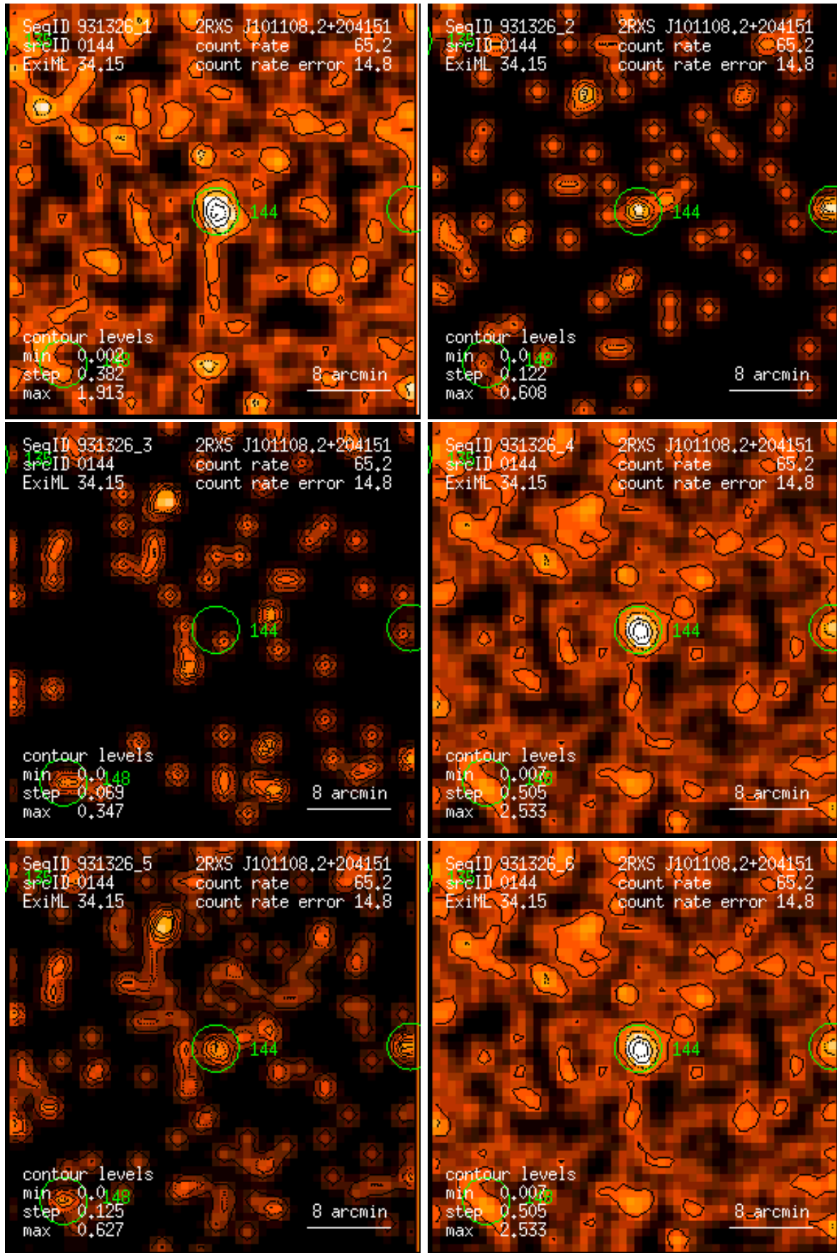
Figure 144: RASS 931326: detection 0144: band rate images, Gaussian filter: (1) PSPC channels 11 – 41, (2) 52 – 90, (3) 91 – 201, (4) 11 – 235, (5) 52 – 201, (6) 11 – 201. Broad band rates in counts/ks. Band rate contour levels in counts/ks/arcmin 2 .
