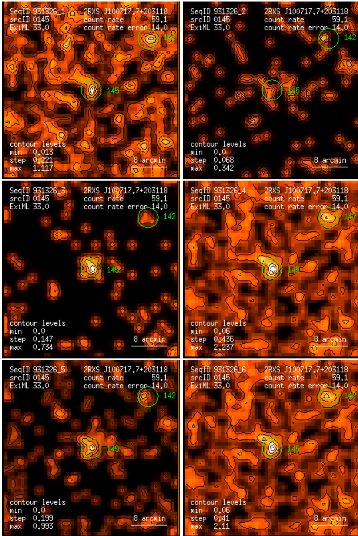
Figure 145: RASS 931326: detection 0145: band rate images, Gaussian filter: (1) PSPC channels 11 – 41, (2) 52 – 90, (3) 91 – 201, (4) 11 – 235, (5) 52 – 201, (6) 11 – 201. Broad band rates in counts/ks. Band rate contour levels in counts/ks/arcmin 2 .
