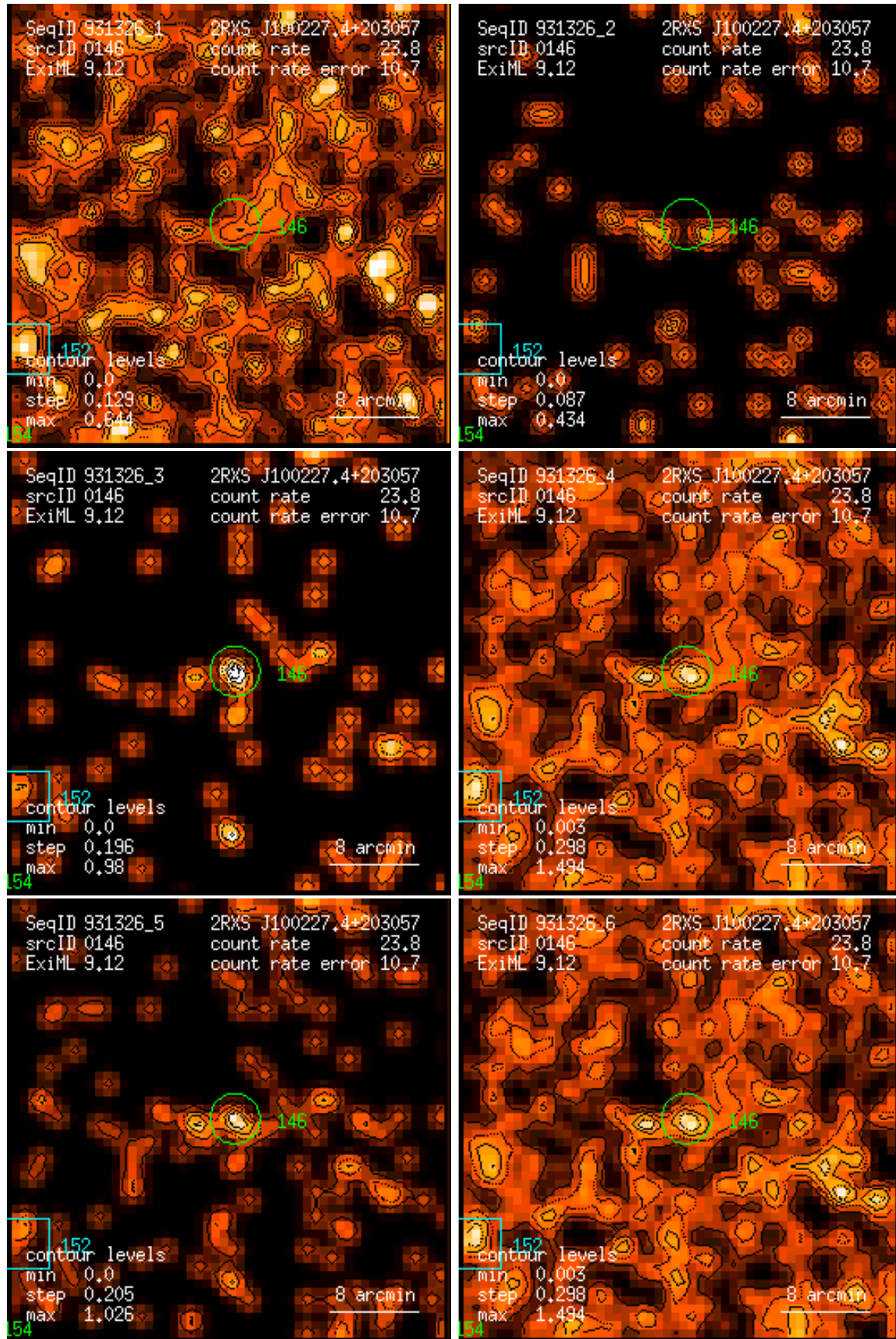
Figure 146: RASS 931326: detection 0146: band rate images, Gaussian filter: (1) PSPC channels 11 – 41, (2) 52 – 90, (3) 91 – 201, (4) 11 – 235, (5) 52 – 201, (6) 11 – 201. Broad band rates in counts/ks. Band rate contour levels in counts/ks/arcmin 2 .
