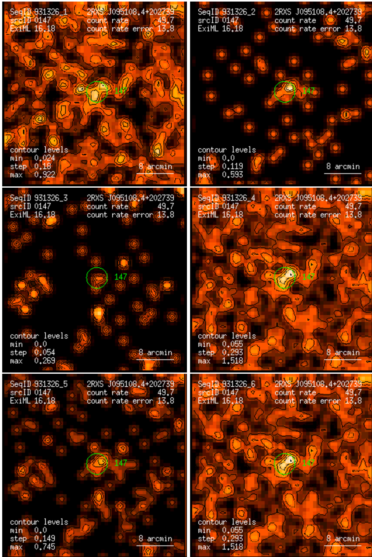
Figure 147: RASS 931326: detection 0147: band rate images, Gaussian filter: (1) PSPC channels 11 – 41, (2) 52 – 90, (3) 91 – 201, (4) 11 – 235, (5) 52 – 201, (6) 11 – 201. Broad band rates in counts/ks. Band rate contour levels in counts/ks/arcmin 2 .
