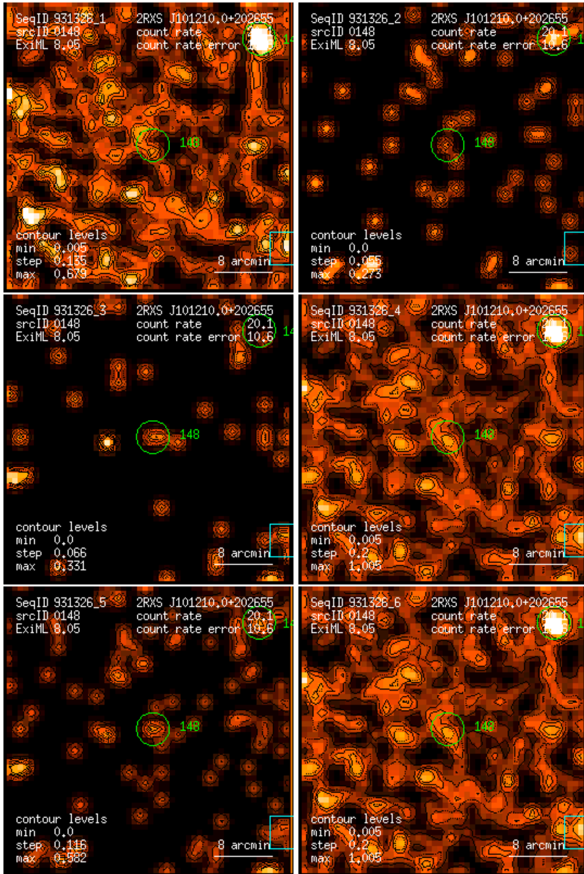
Figure 148: RASS 931326: detection 0148: band rate images, Gaussian filter: (1) PSPC channels 11 – 41, (2) 52 – 90, (3) 91 – 201, (4) 11 – 235, (5) 52 – 201, (6) 11 – 201. Broad band rates in counts/ks. Band rate contour levels in counts/ks/arcmin 2 .
