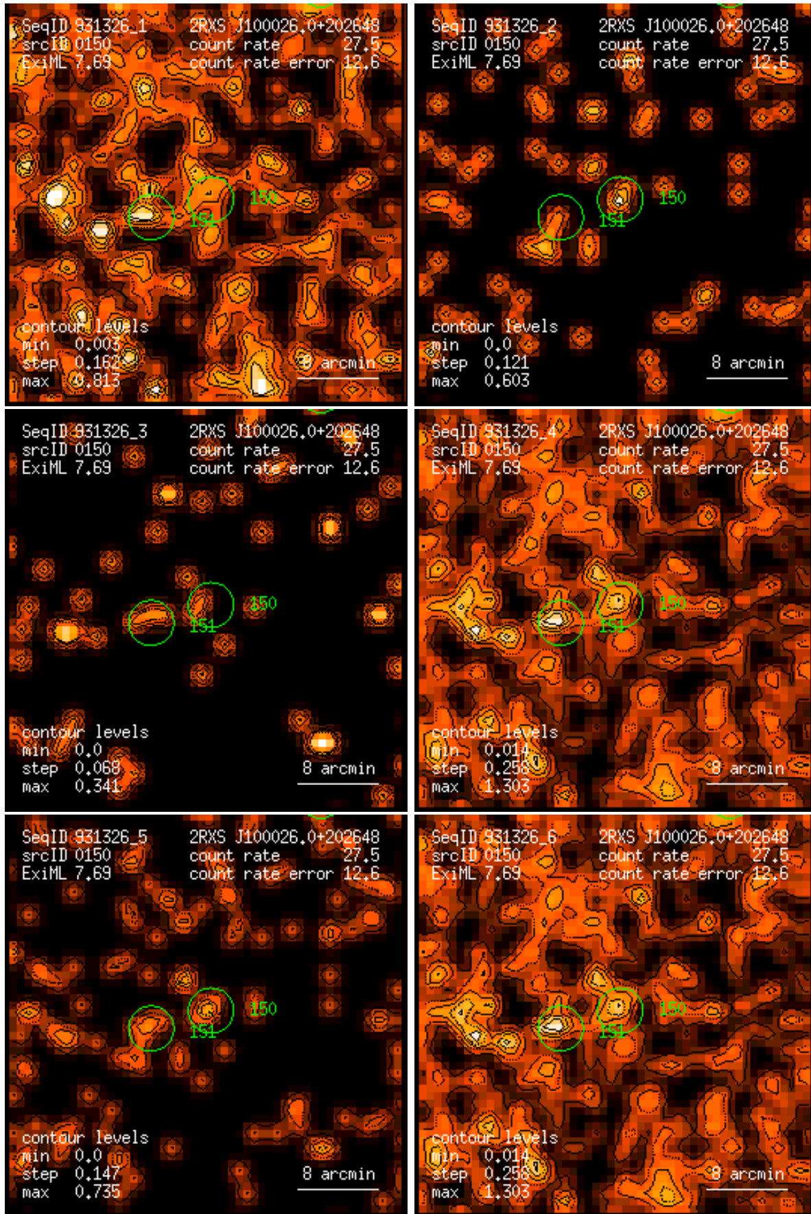
Figure 150: RASS 931326: detection 0150: band rate images, Gaussian filter: (1) PSPC channels 11 – 41, (2) 52 – 90, (3) 91 – 201, (4) 11 – 235, (5) 52 – 201, (6) 11 – 201. Broad band rates in counts/ks. Band rate contour levels in counts/ks/arcmin 2 .
