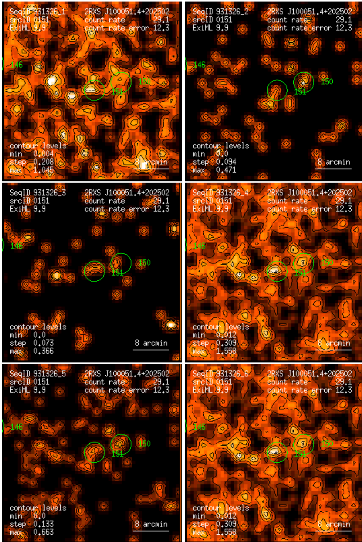
Figure 151: RASS 931326: detection 0151: band rate images, Gaussian filter: (1) PSPC channels 11 – 41, (2) 52 – 90, (3) 91 – 201, (4) 11 – 235, (5) 52 – 201, (6) 11 – 201. Broad band rates in counts/ks. Band rate contour levels in counts/ks/arcmin 2 .
