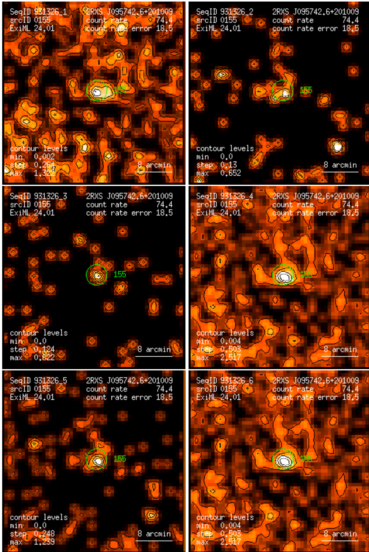
Figure 155: RASS 931326: detection 0155: band rate images, Gaussian filter: (1) PSPC channels 11 – 41, (2) 52 – 90, (3) 91 – 201, (4) 11 – 235, (5) 52 – 201, (6) 11 – 201. Broad band rates in counts/ks. Band rate contour levels in counts/ks/arcmin 2 .
