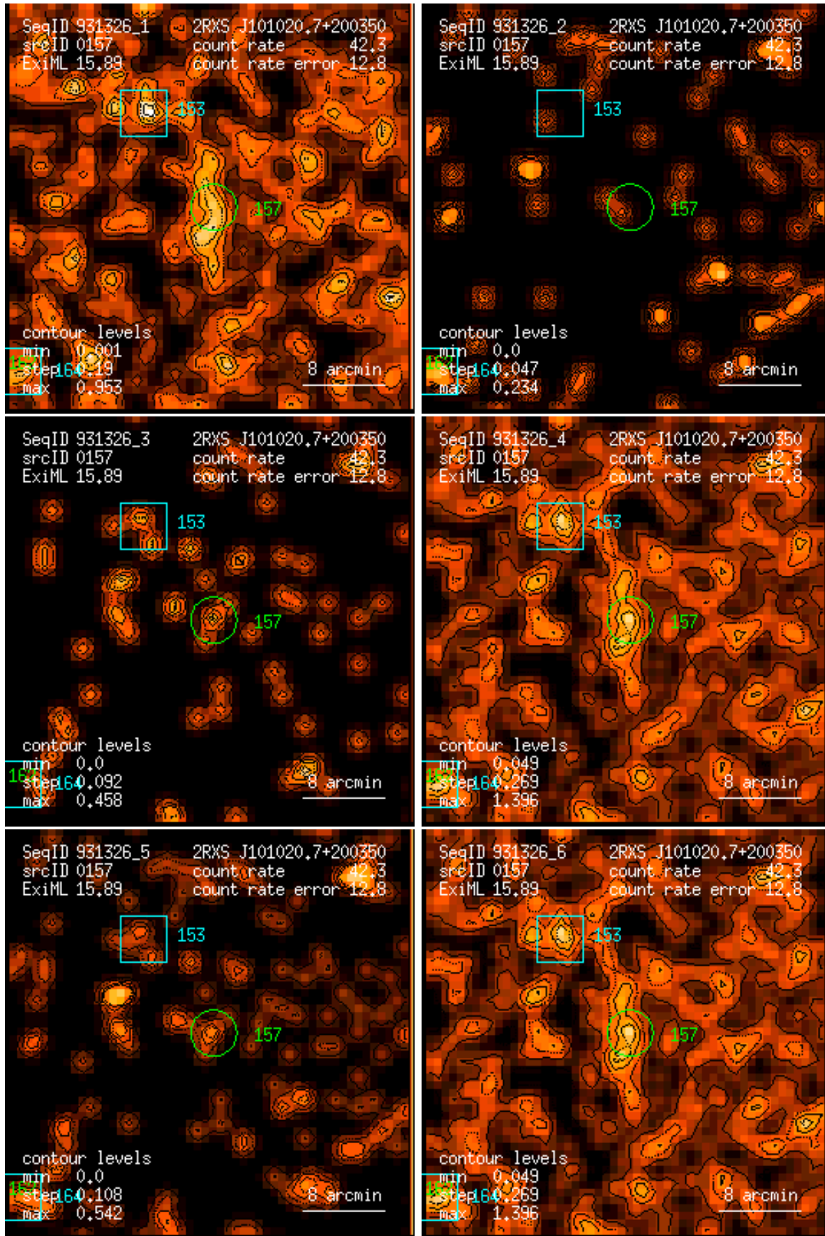
Figure 157: RASS 931326: detection 0157: band rate images, Gaussian filter: (1) PSPC channels 11 – 41, (2) 52 – 90, (3) 91 – 201, (4) 11 – 235, (5) 52 – 201, (6) 11 – 201. Broad band rates in counts/ks. Band rate contour levels in counts/ks/arcmin 2 .
