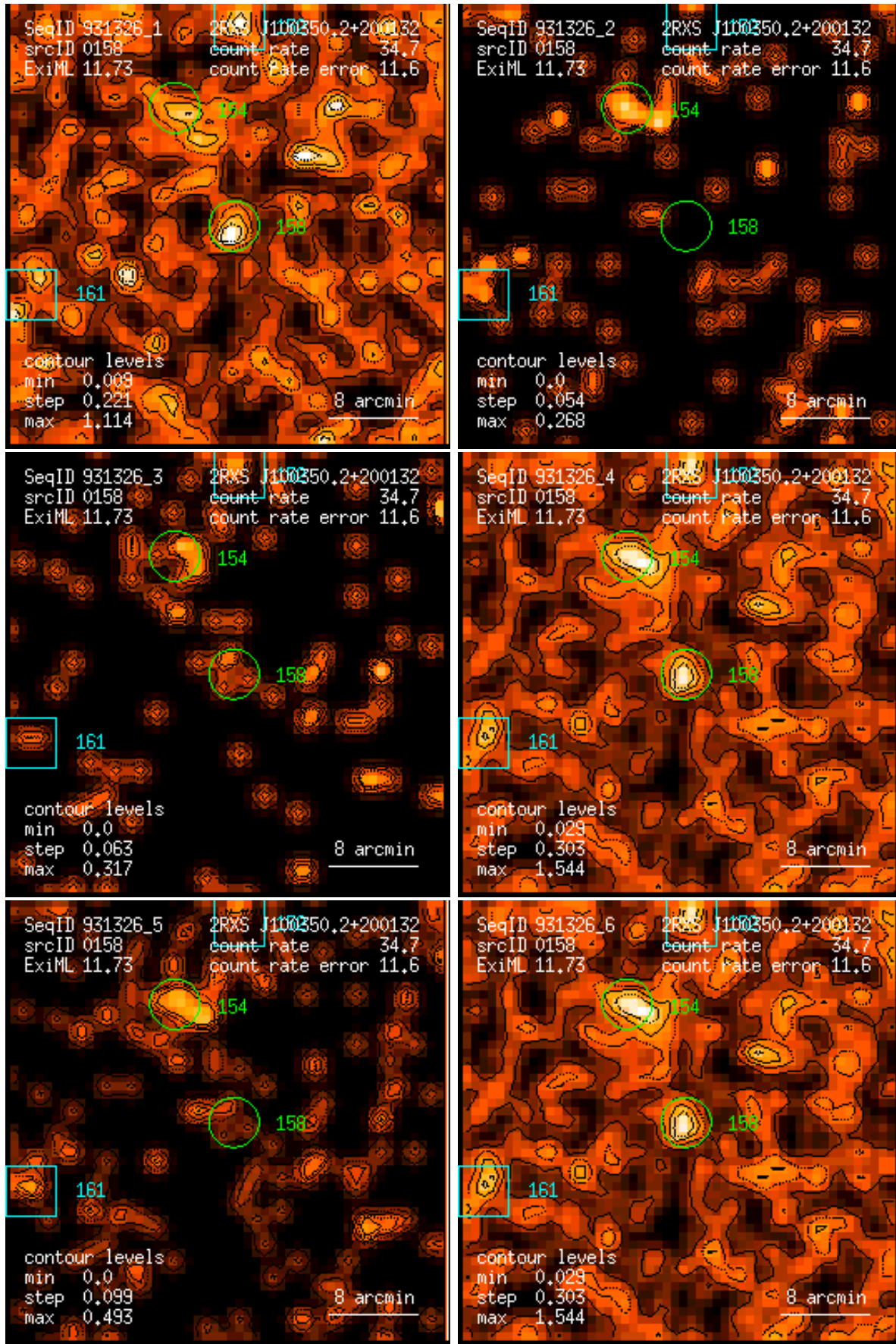
Figure 158: RASS 931326: detection 0158: band rate images, Gaussian filter: (1) PSPC channels 11 – 41, (2) 52 – 90, (3) 91 – 201, (4) 11 – 235, (5) 52 – 201, (6) 11 – 201. Broad band rates in counts/ks. Band rate contour levels in counts/ks/arcmin 2 .
