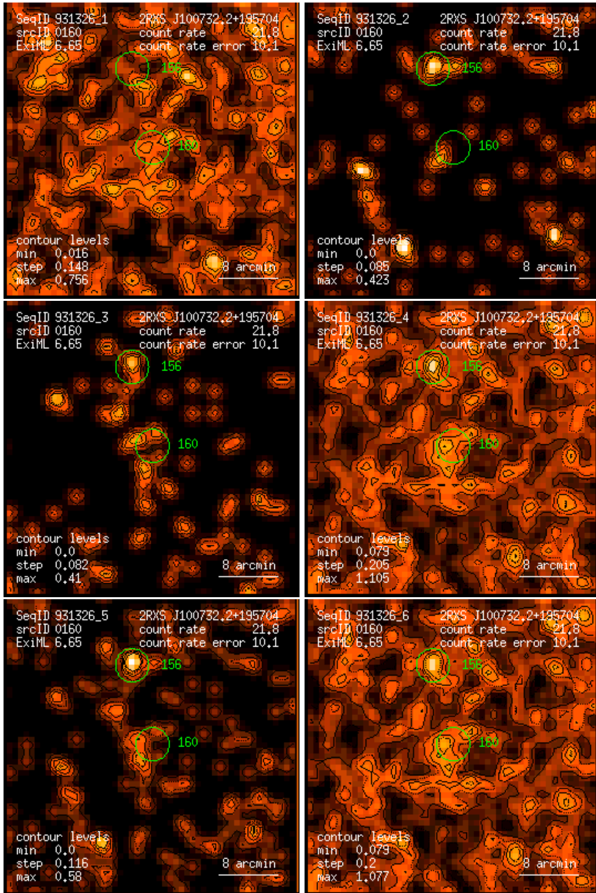
Figure 160: RASS 931326: detection 0160: band rate images, Gaussian filter: (1) PSPC channels 11 – 41, (2) 52 – 90, (3) 91 – 201, (4) 11 – 235, (5) 52 – 201, (6) 11 – 201. Broad band rates in counts/ks. Band rate contour levels in counts/ks/arcmin 2 .
