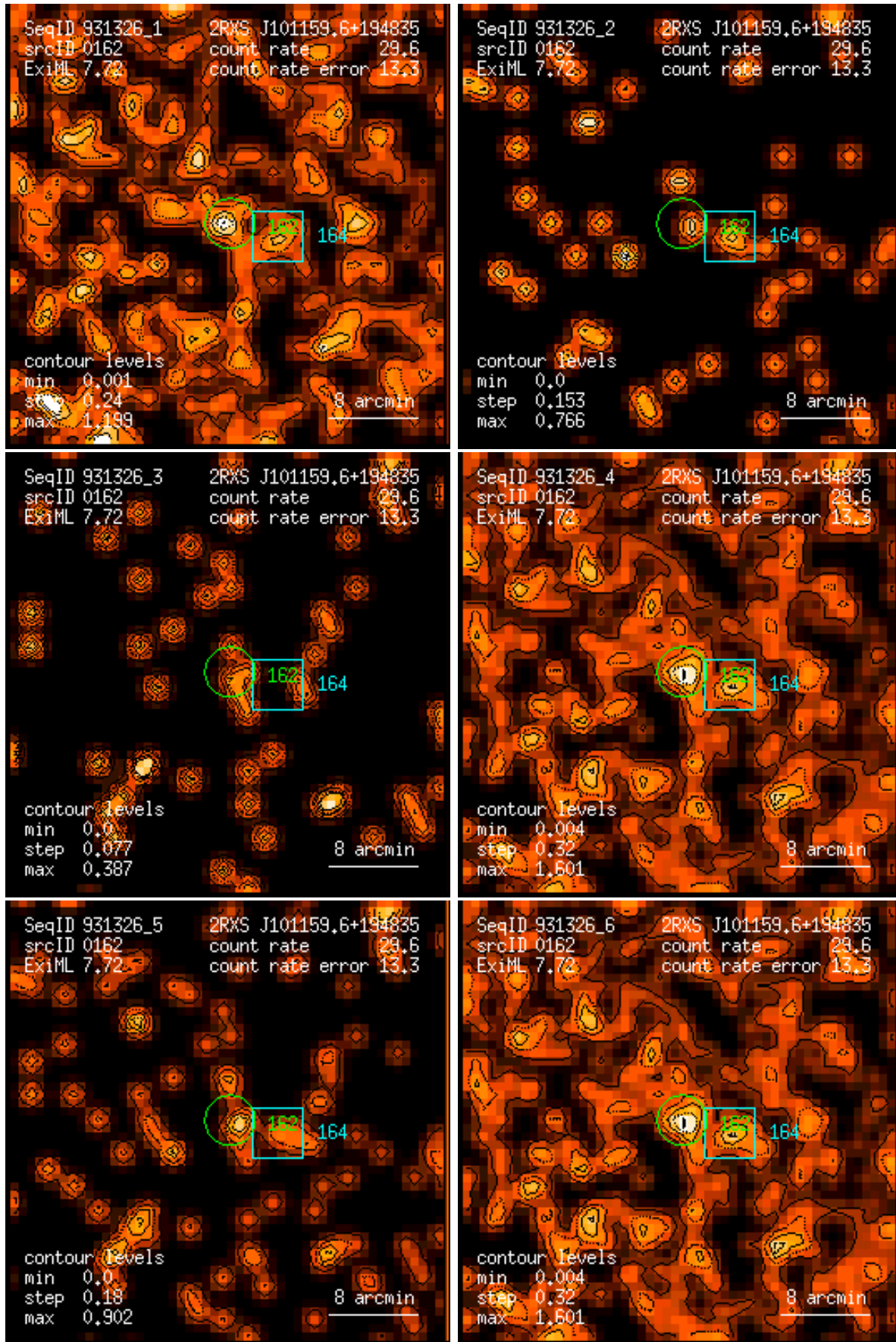
Figure 162: RASS 931326: detection 0162: band rate images, Gaussian filter: (1) PSPC channels 11 – 41, (2) 52 – 90, (3) 91 – 201, (4) 11 – 235, (5) 52 – 201, (6) 11 – 201. Broad band rates in counts/ks. Band rate contour levels in counts/ks/arcmin 2 .
