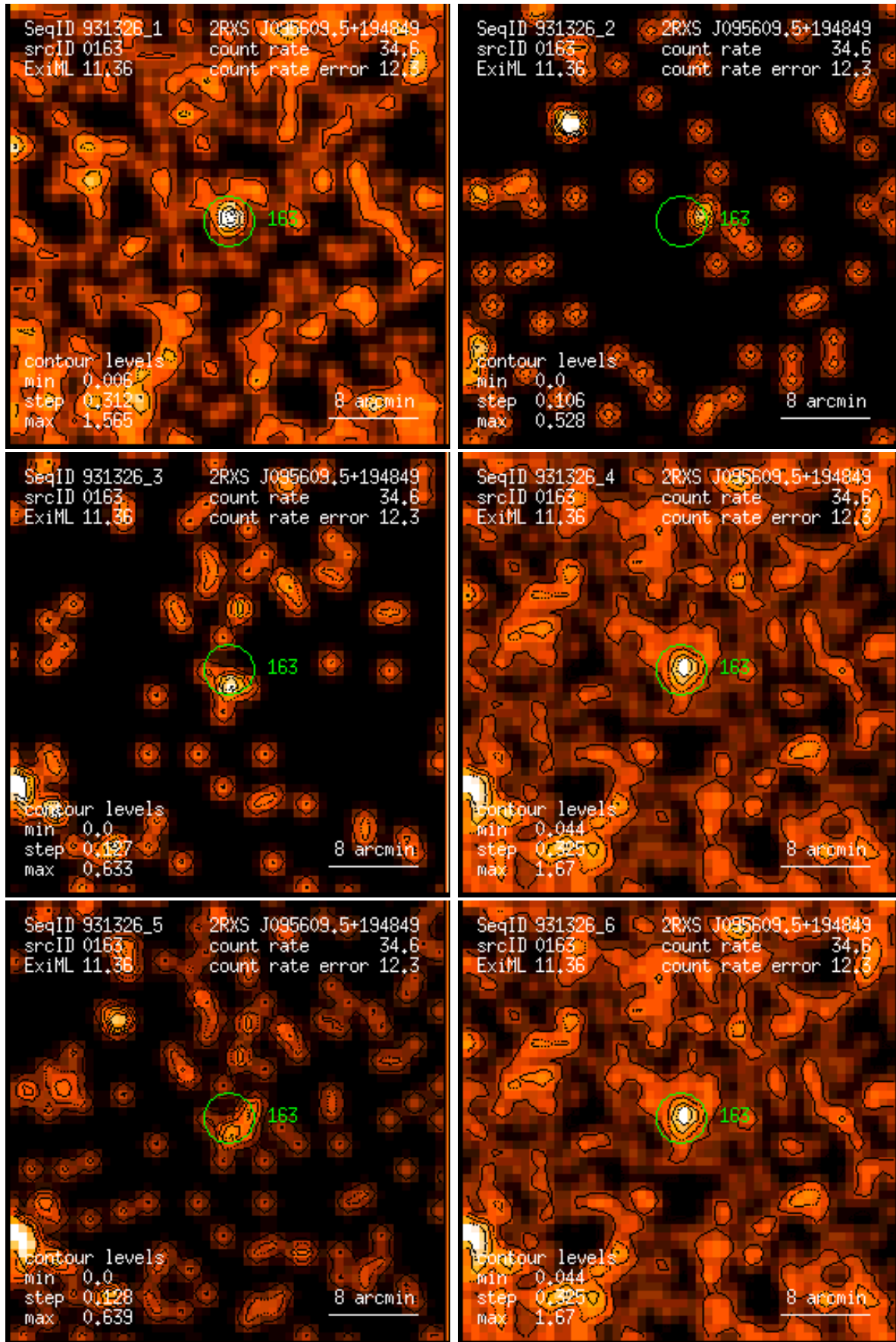
Figure 163: RASS 931326: detection 0163: band rate images, Gaussian filter: (1) PSPC channels 11 – 41, (2) 52 – 90, (3) 91 – 201, (4) 11 – 235, (5) 52 – 201, (6) 11 – 201. Broad band rates in counts/ks. Band rate contour levels in counts/ks/arcmin 2 .
