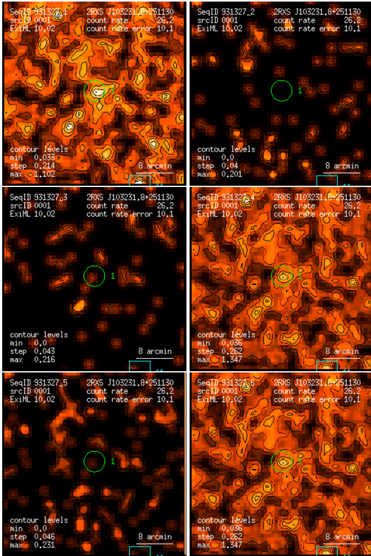
Figure 1: RASS 931327: detection 0001: band rate images, Gaussian filter: (1) PSPC channels 11 – 41, (2) 52 – 90, (3) 91 – 201, (4) 11 – 235, (5) 52 – 201, (6) 11 – 201. Broad band rates in counts/ks. Band rate contour levels in counts/ks/arcmin 2 .
