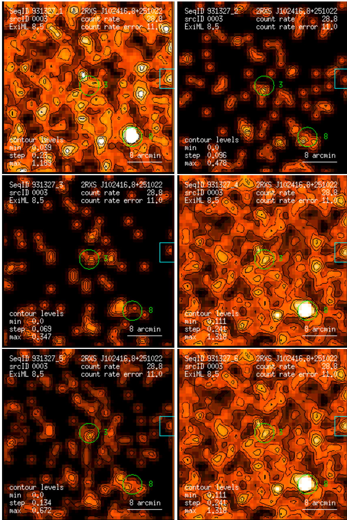
Figure 3: RASS 931327: detection 0003: band rate images, Gaussian filter: (1) PSPC channels 11 – 41, (2) 52 – 90, (3) 91 – 201, (4) 11 – 235, (5) 52 – 201, (6) 11 – 201. Broad band rates in counts/ks. Band rate contour levels in counts/ks/arcmin 2 .
