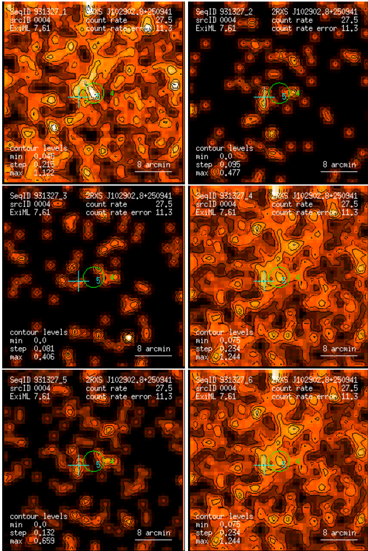
Figure 4: RASS 931327: detection 0004: band rate images, Gaussian filter: (1) PSPC channels 11 – 41, (2) 52 – 90, (3) 91 – 201, (4) 11 – 235, (5) 52 – 201, (6) 11 – 201. Broad band rates in counts/ks. Band rate contour levels in counts/ks/arcmin 2 .
