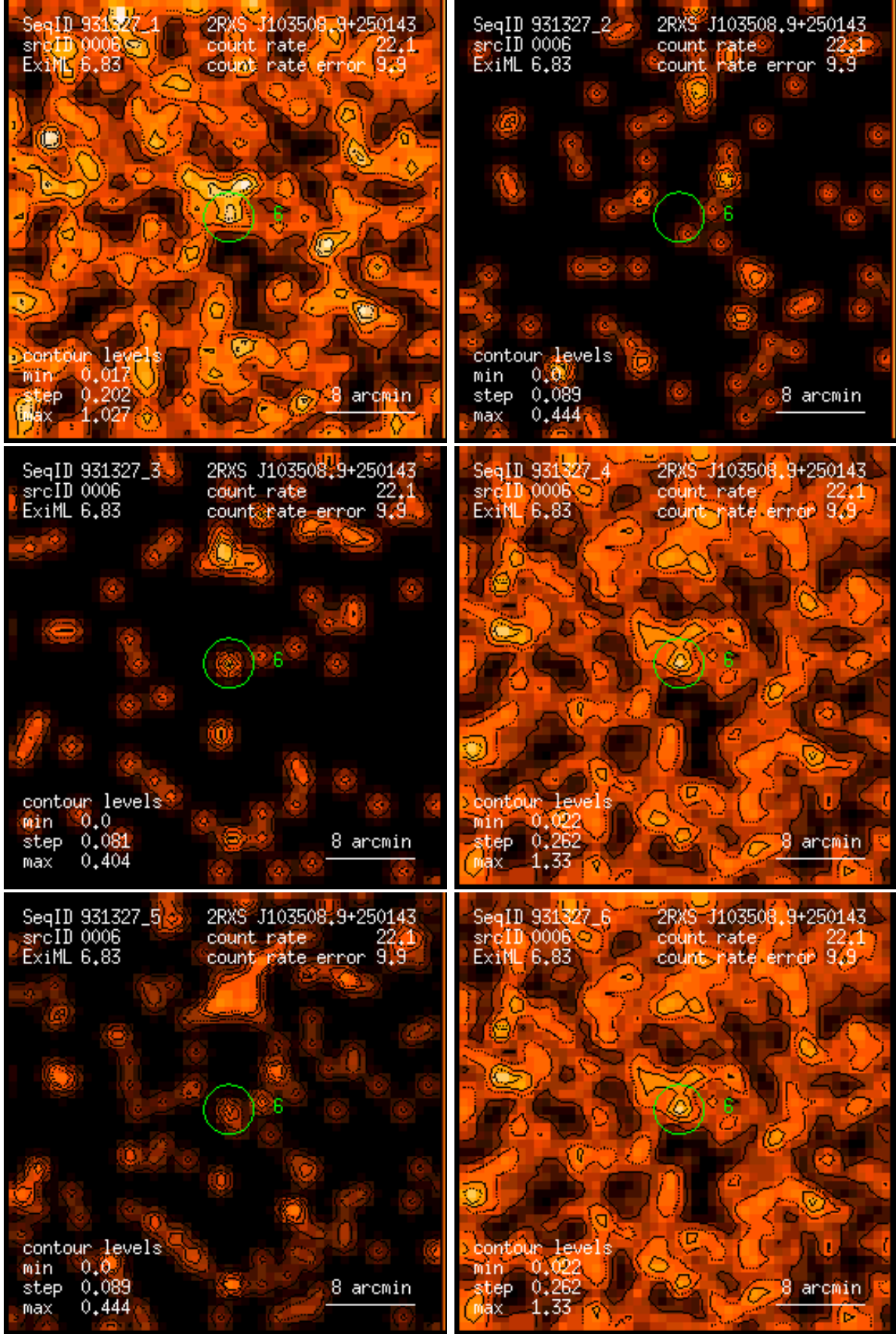
Figure 6: RASS 931327: detection 0006: band rate images, Gaussian filter: (1) PSPC channels 11 – 41, (2) 52 – 90, (3) 91 – 201, (4) 11 – 235, (5) 52 – 201, (6) 11 – 201. Broad band rates in counts/ks. Band rate contour levels in counts/ks/arcmin 2 .
