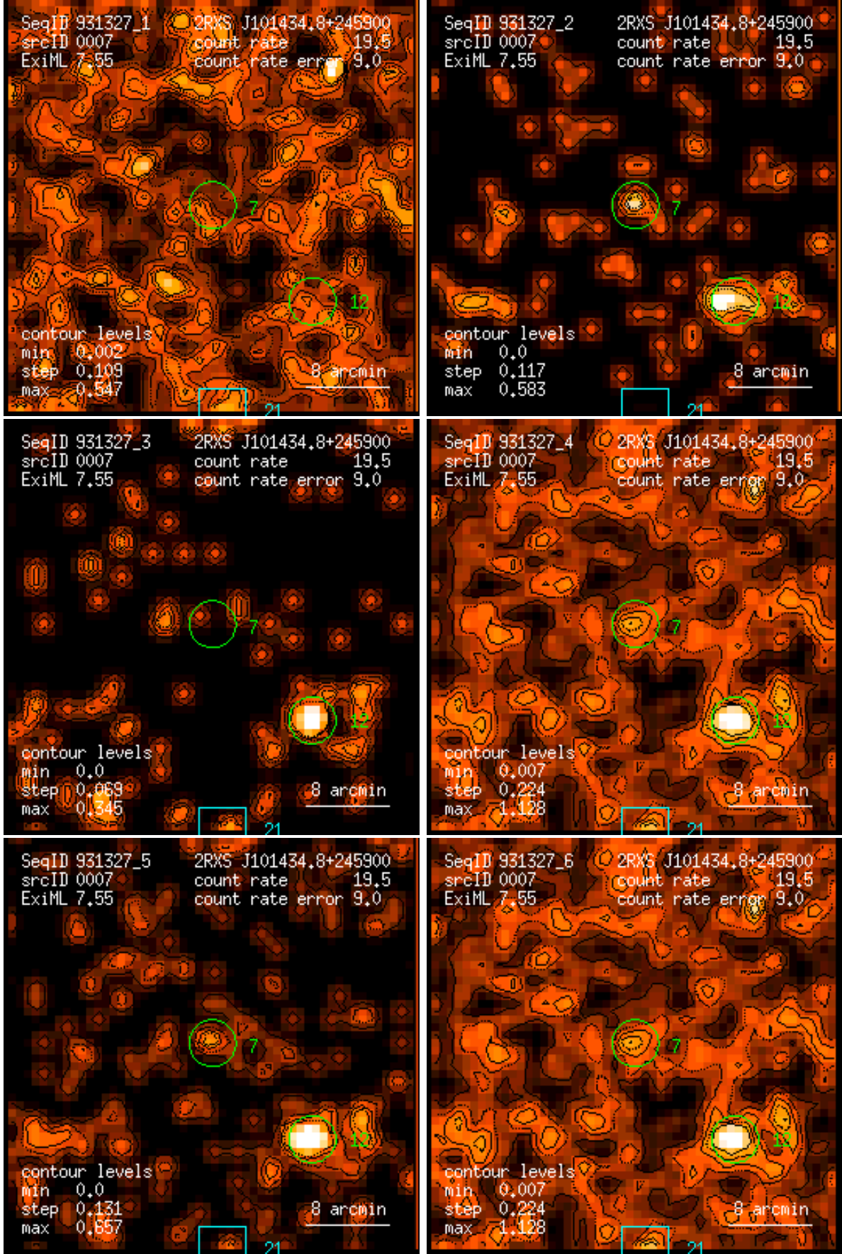
Figure 7: RASS 931327: detection 0007: band rate images, Gaussian filter: (1) PSPC channels 11 – 41, (2) 52 – 90, (3) 91 – 201, (4) 11 – 235, (5) 52 – 201, (6) 11 – 201. Broad band rates in counts/ks. Band rate contour levels in counts/ks/arcmin 2 .
