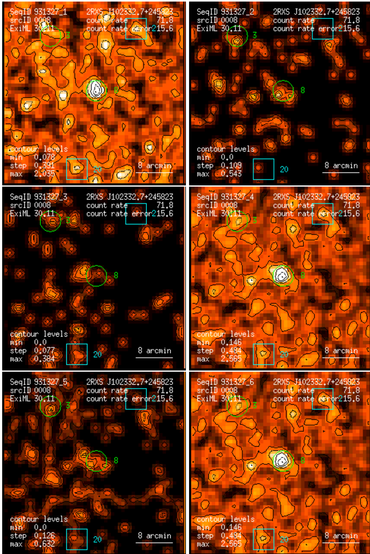
Figure 8: RASS 931327: detection 0008: band rate images, Gaussian filter: (1) PSPC channels 11 – 41, (2) 52 – 90, (3) 91 – 201, (4) 11 – 235, (5) 52 – 201, (6) 11 – 201. Broad band rates in counts/ks. Band rate contour levels in counts/ks/arcmin 2 .
