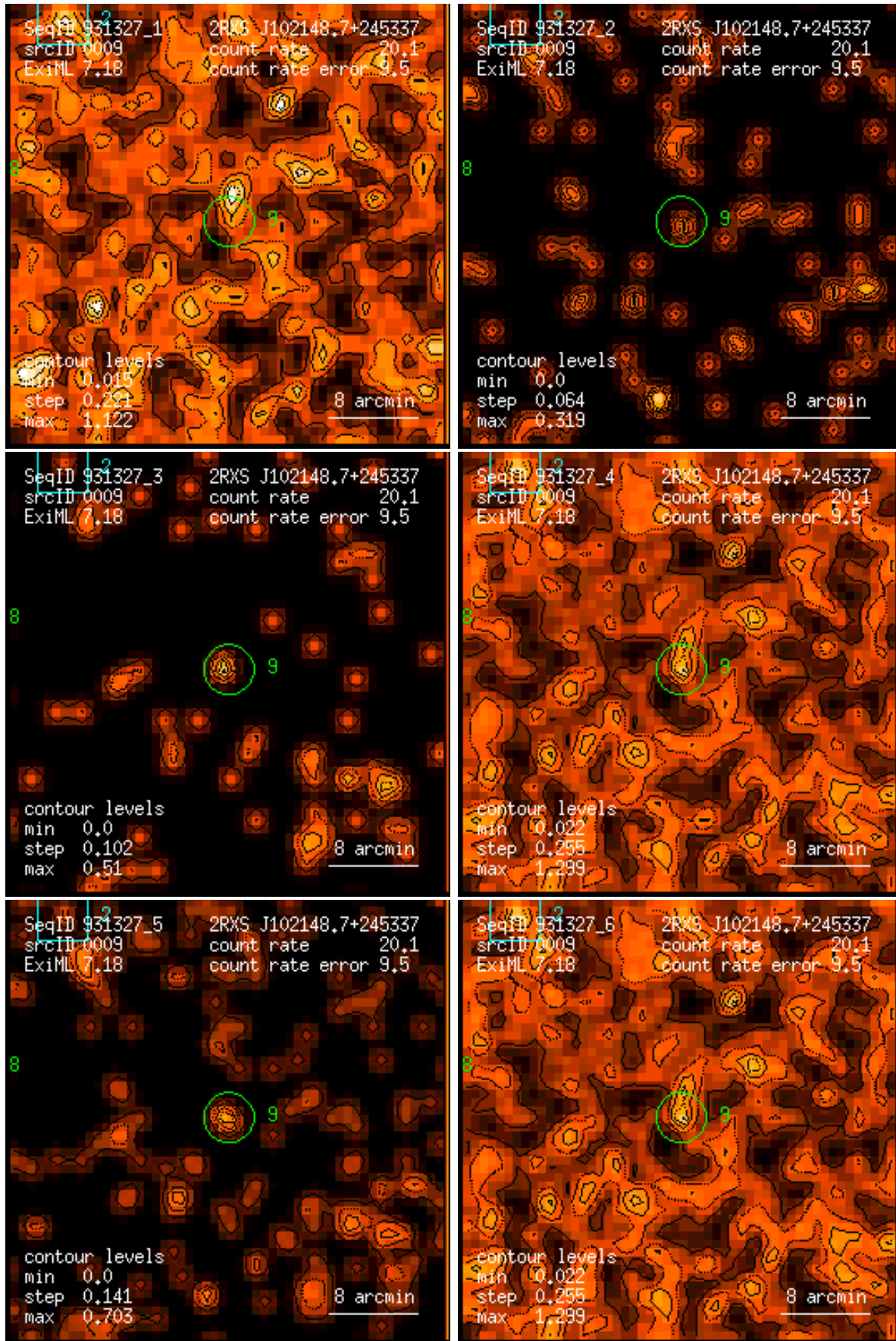
Figure 9: RASS 931327: detection 0009: band rate images, Gaussian filter: (1) PSPC channels 11 – 41, (2) 52 – 90, (3) 91 – 201, (4) 11 – 235, (5) 52 – 201, (6) 11 – 201. Broad band rates in counts/ks. Band rate contour levels in counts/ks/arcmin 2 .
