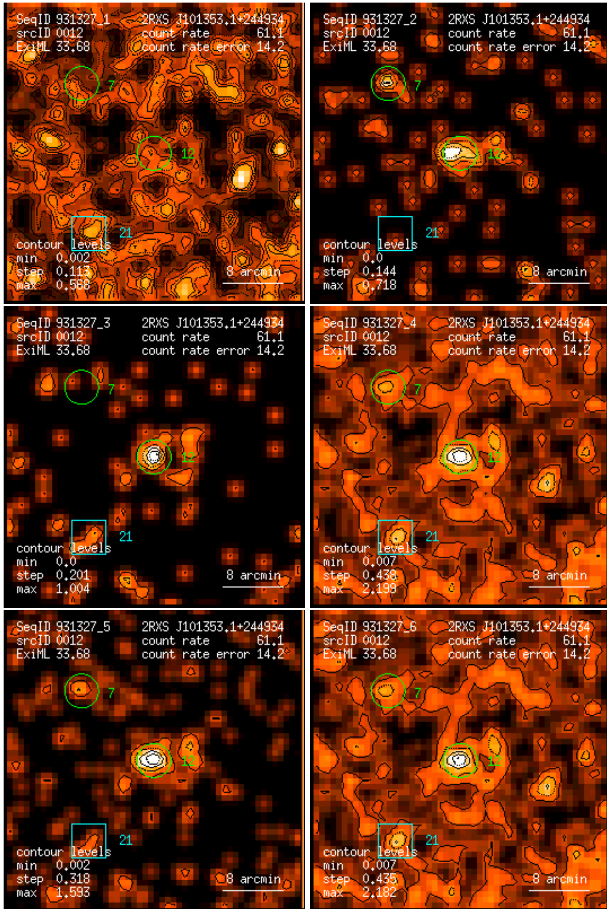
Figure 12: RASS 931327: detection 0012: band rate images, Gaussian filter: (1) PSPC channels 11 – 41, (2) 52 – 90, (3) 91 – 201, (4) 11 – 235, (5) 52 – 201, (6) 11 – 201. Broad band rates in counts/ks. Band rate contour levels in counts/ks/arcmin 2 .
