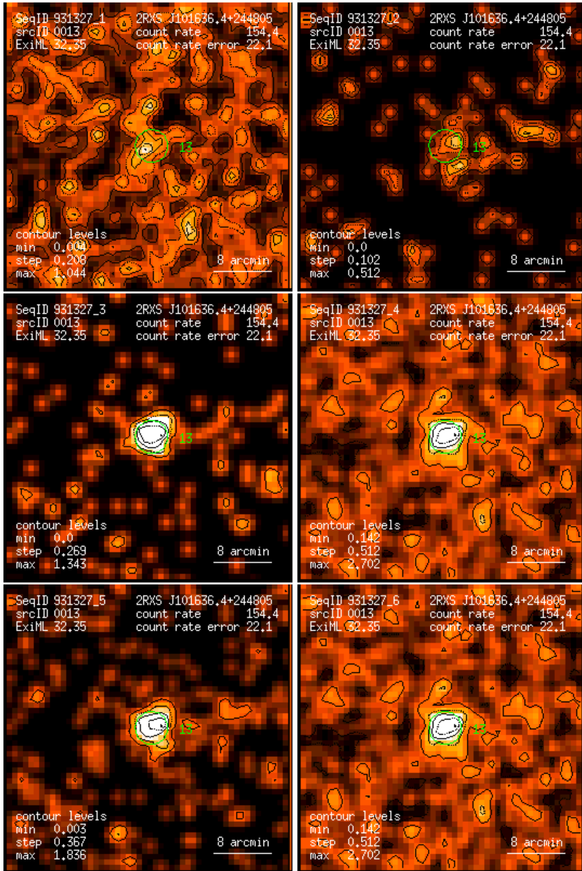
Figure 13: RASS 931327: detection 0013: band rate images, Gaussian filter: (1) PSPC channels 11 – 41, (2) 52 – 90, (3) 91 – 201, (4) 11 – 235, (5) 52 – 201, (6) 11 – 201. Broad band rates in counts/ks. Band rate contour levels in counts/ks/arcmin 2 .
