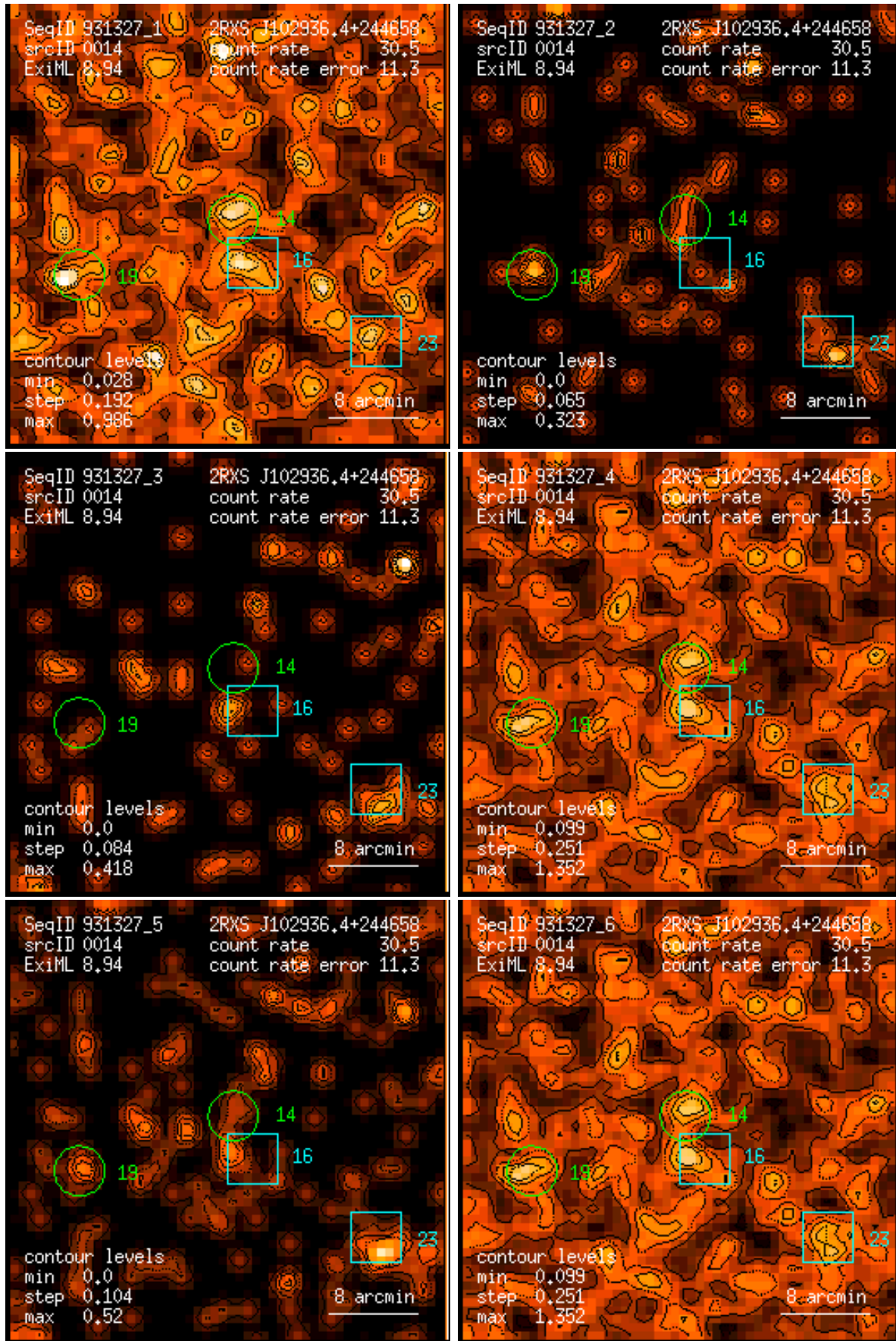
Figure 14: RASS 931327: detection 0014: band rate images, Gaussian filter: (1) PSPC channels 11 – 41, (2) 52 – 90, (3) 91 – 201, (4) 11 – 235, (5) 52 – 201, (6) 11 – 201. Broad band rates in counts/ks. Band rate contour levels in counts/ks/arcmin 2 .
