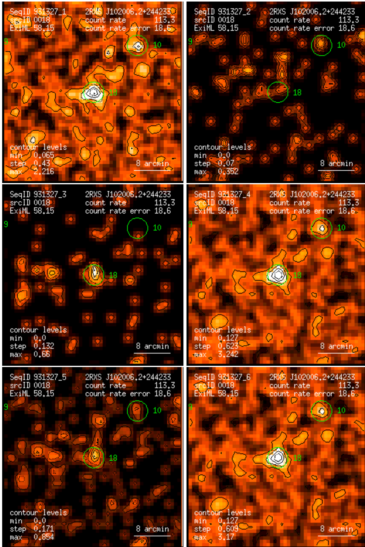
Figure 18: RASS 931327: detection 0018: band rate images, Gaussian filter: (1) PSPC channels 11 – 41, (2) 52 – 90, (3) 91 – 201, (4) 11 – 235, (5) 52 – 201, (6) 11 – 201. Broad band rates in counts/ks. Band rate contour levels in counts/ks/arcmin 2 .
