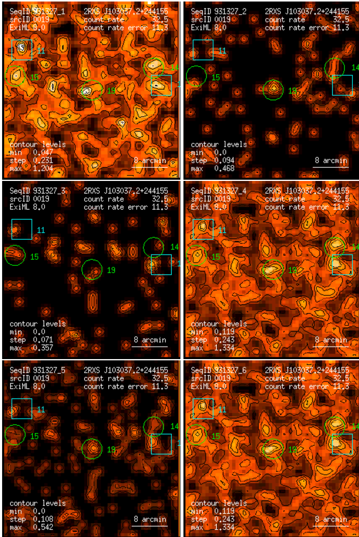
Figure 19: RASS 931327: detection 0019: band rate images, Gaussian filter: (1) PSPC channels 11 – 41, (2) 52 – 90, (3) 91 – 201, (4) 11 – 235, (5) 52 – 201, (6) 11 – 201. Broad band rates in counts/ks. Band rate contour levels in counts/ks/arcmin 2 .
