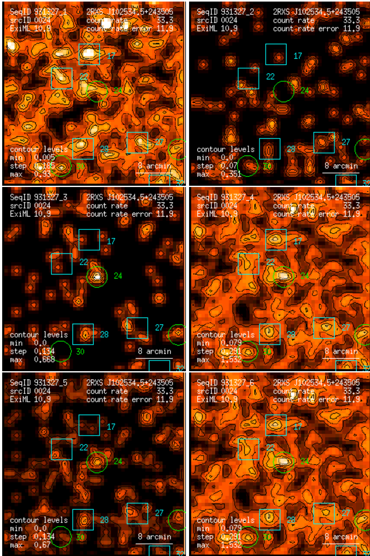
Figure 24: RASS 931327: detection 0024: band rate images, Gaussian filter: (1) PSPC channels 11 – 41, (2) 52 – 90, (3) 91 – 201, (4) 11 – 235, (5) 52 – 201, (6) 11 – 201. Broad band rates in counts/ks. Band rate contour levels in counts/ks/arcmin 2 .
