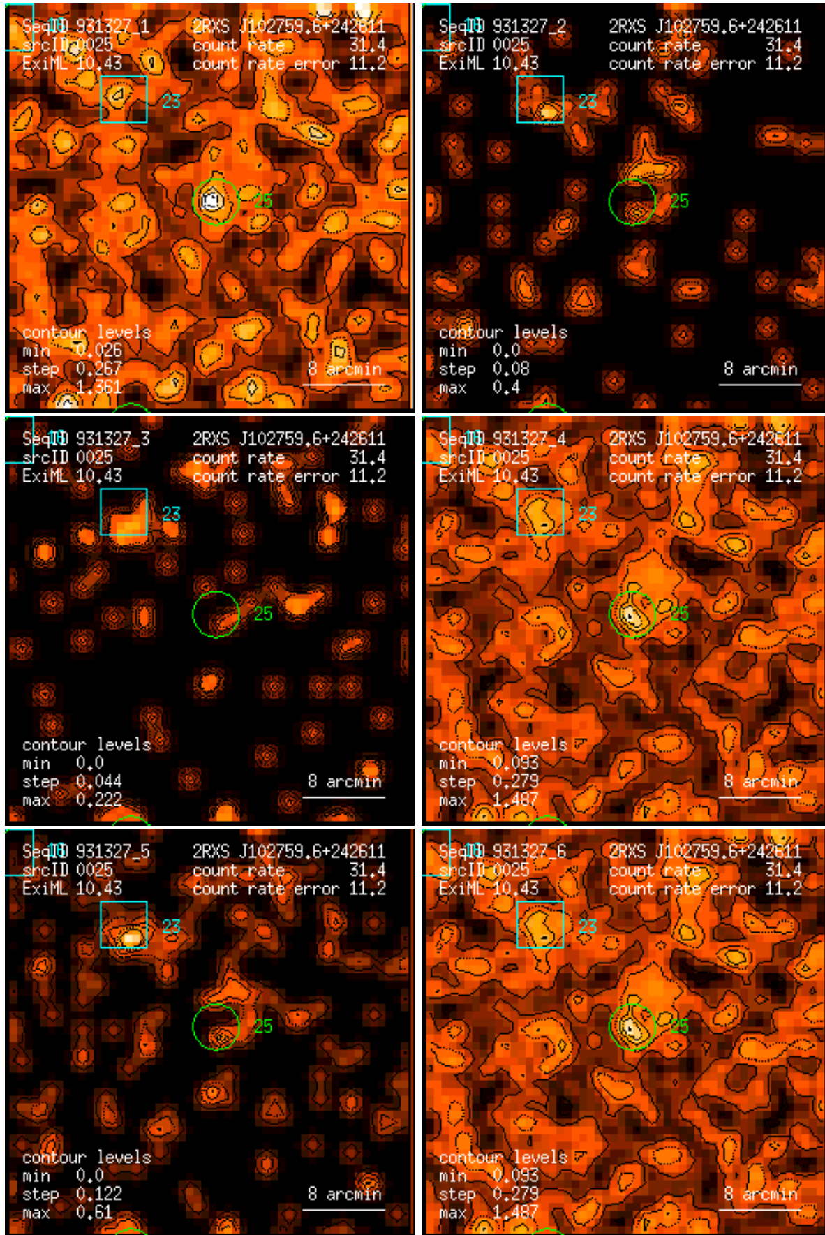
Figure 25: RASS 931327: detection 0025: band rate images, Gaussian filter: (1) PSPC channels 11 – 41, (2) 52 – 90, (3) 91 – 201, (4) 11 – 235, (5) 52 – 201, (6) 11 – 201. Broad band rates in counts/ks. Band rate contour levels in counts/ks/arcmin 2 .
