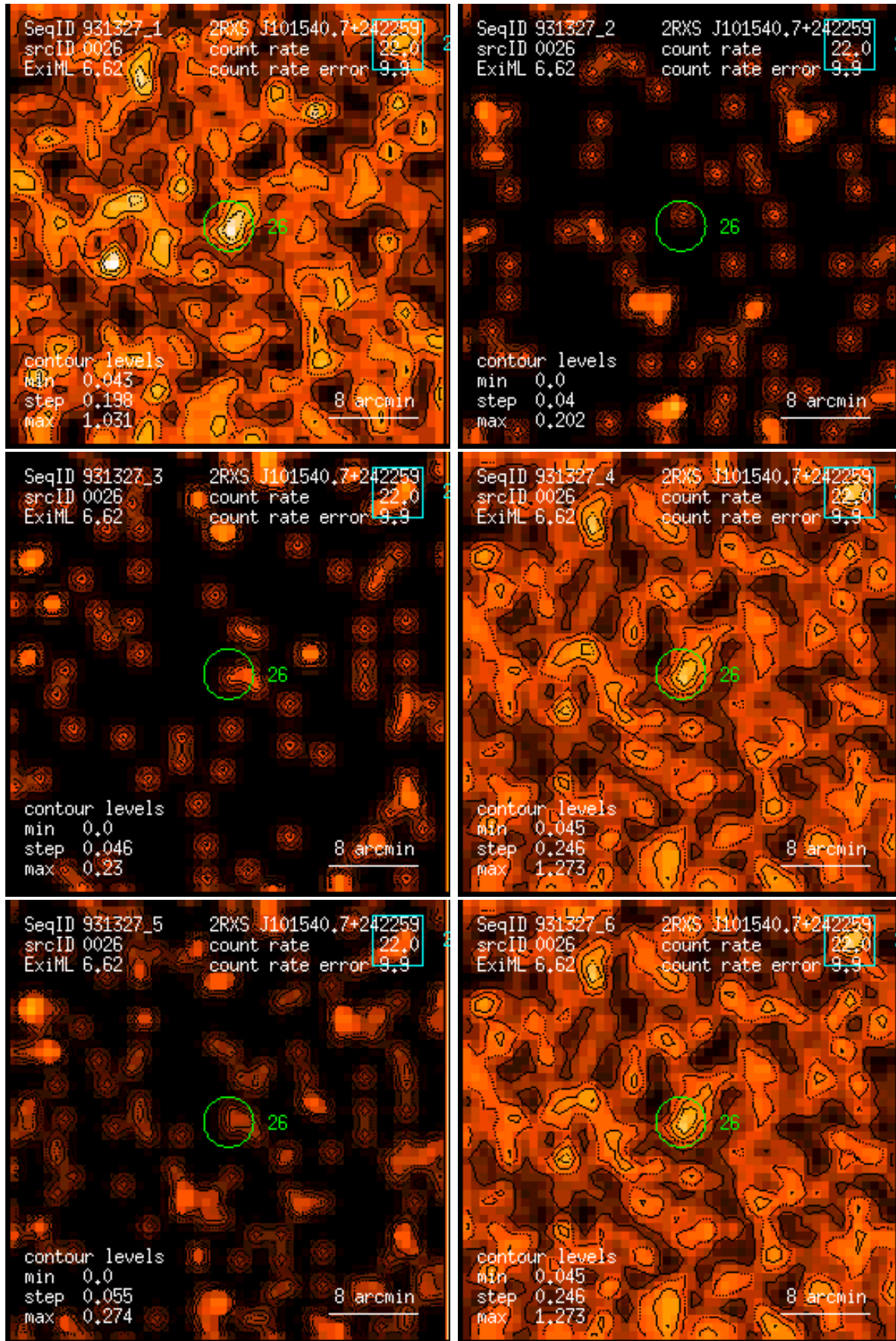
Figure 26: RASS 931327: detection 0026: band rate images, Gaussian filter: (1) PSPC channels 11 – 41, (2) 52 – 90, (3) 91 – 201, (4) 11 – 235, (5) 52 – 201, (6) 11 – 201. Broad band rates in counts/ks. Band rate contour levels in counts/ks/arcmin 2 .
