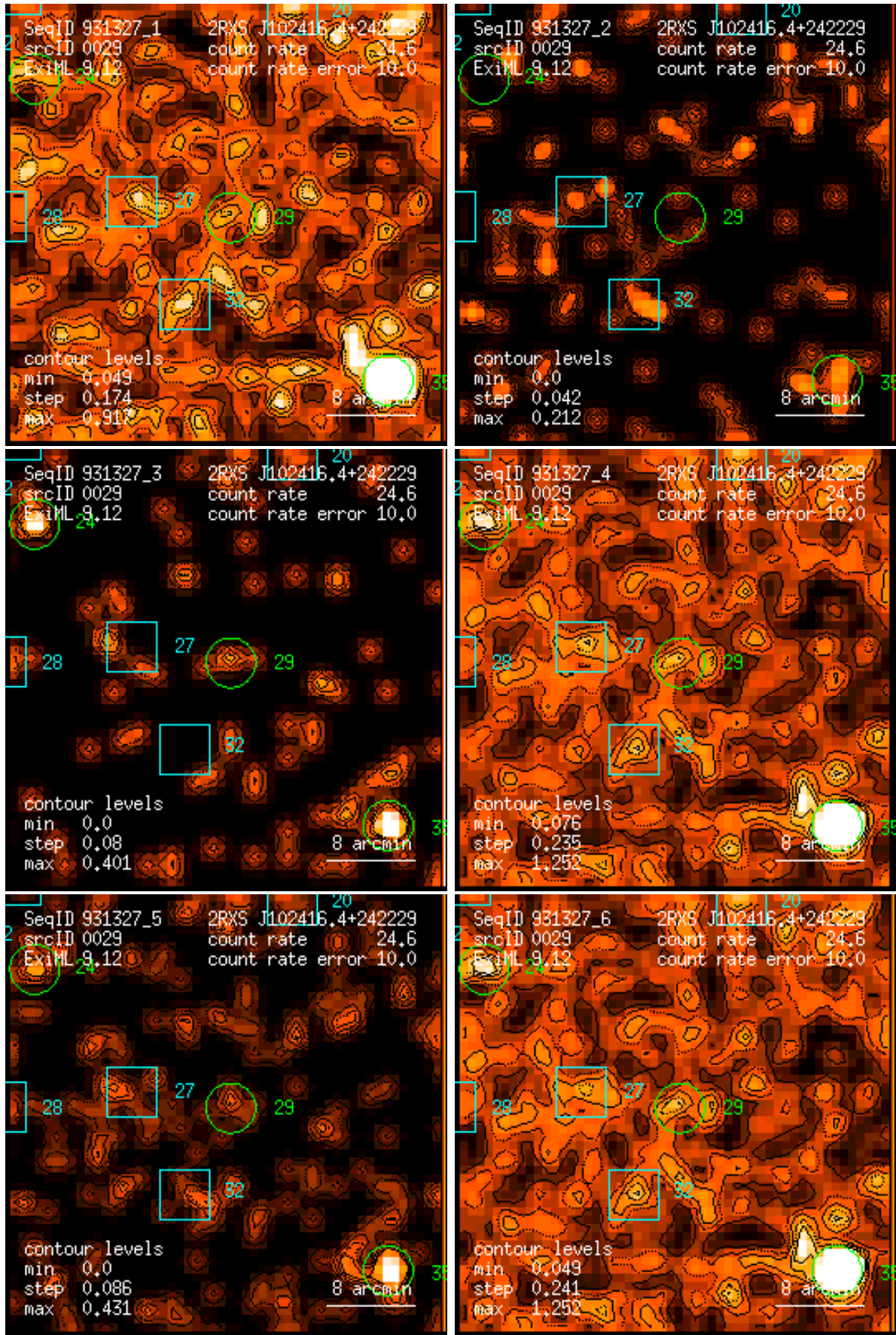
Figure 29: RASS 931327: detection 0029: band rate images, Gaussian filter: (1) PSPC channels 11 – 41, (2) 52 – 90, (3) 91 – 201, (4) 11 – 235, (5) 52 – 201, (6) 11 – 201. Broad band rates in counts/ks. Band rate contour levels in counts/ks/arcmin 2 .
