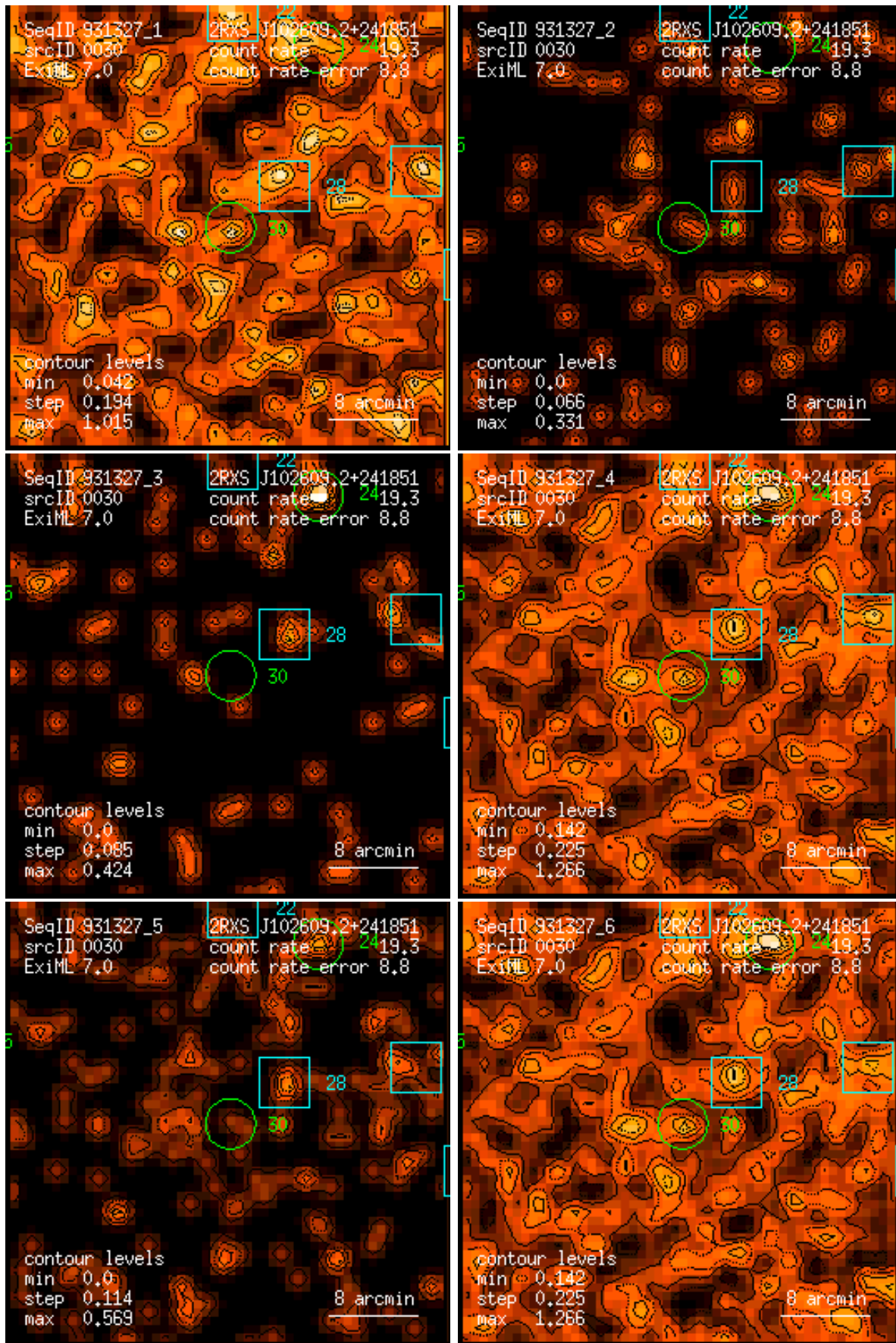
Figure 30: RASS 931327: detection 0030: band rate images, Gaussian filter: (1) PSPC channels 11 – 41, (2) 52 – 90, (3) 91 – 201, (4) 11 – 235, (5) 52 – 201, (6) 11 – 201. Broad band rates in counts/ks. Band rate contour levels in counts/ks/arcmin 2 .
