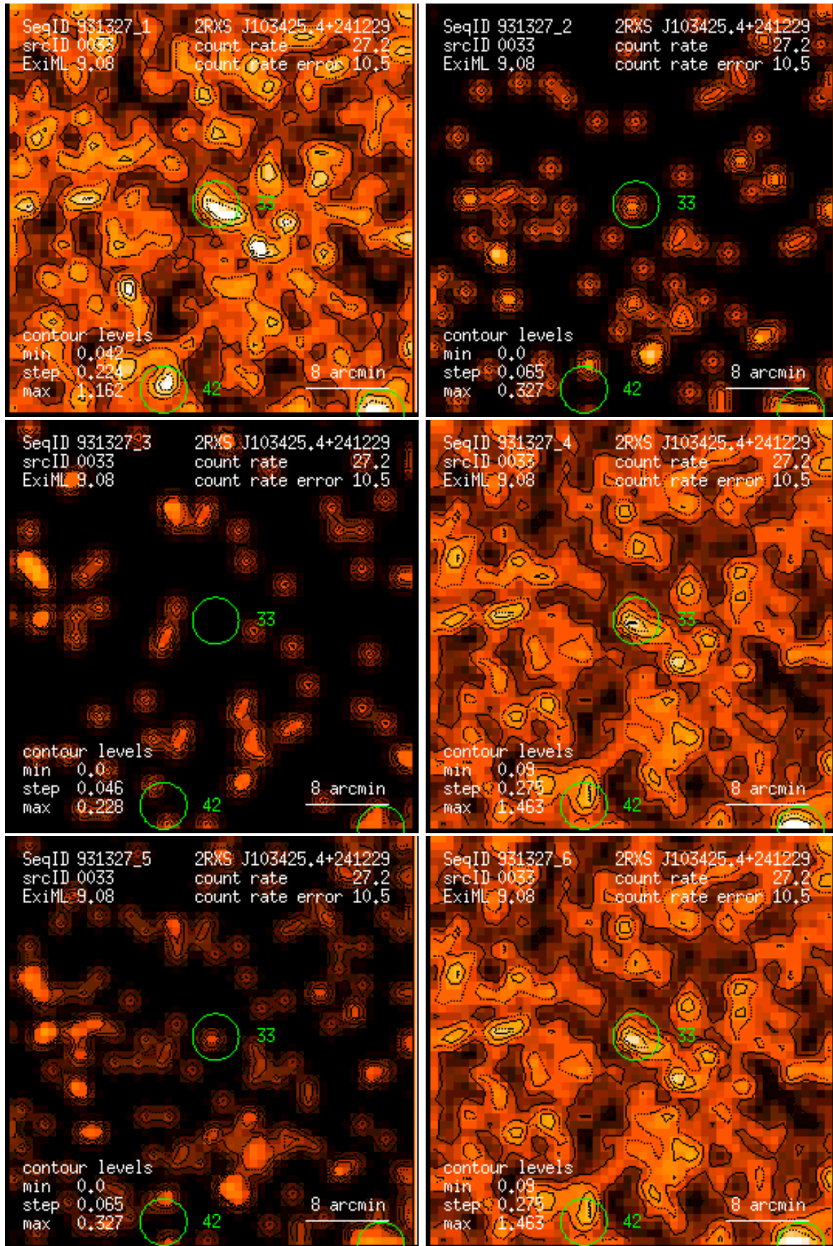
Figure 33: RASS 931327: detection 0033: band rate images, Gaussian filter: (1) PSPC channels 11 – 41, (2) 52 – 90, (3) 91 – 201, (4) 11 – 235, (5) 52 – 201, (6) 11 – 201. Broad band rates in counts/ks. Band rate contour levels in counts/ks/arcmin 2 .
