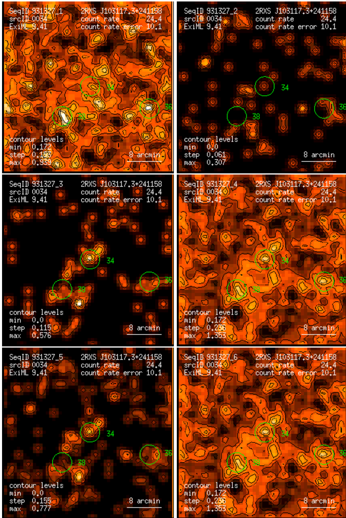
Figure 34: RASS 931327: detection 0034: band rate images, Gaussian filter: (1) PSPC channels 11 – 41, (2) 52 – 90, (3) 91 – 201, (4) 11 – 235, (5) 52 – 201, (6) 11 – 201. Broad band rates in counts/ks. Band rate contour levels in counts/ks/arcmin 2 .
