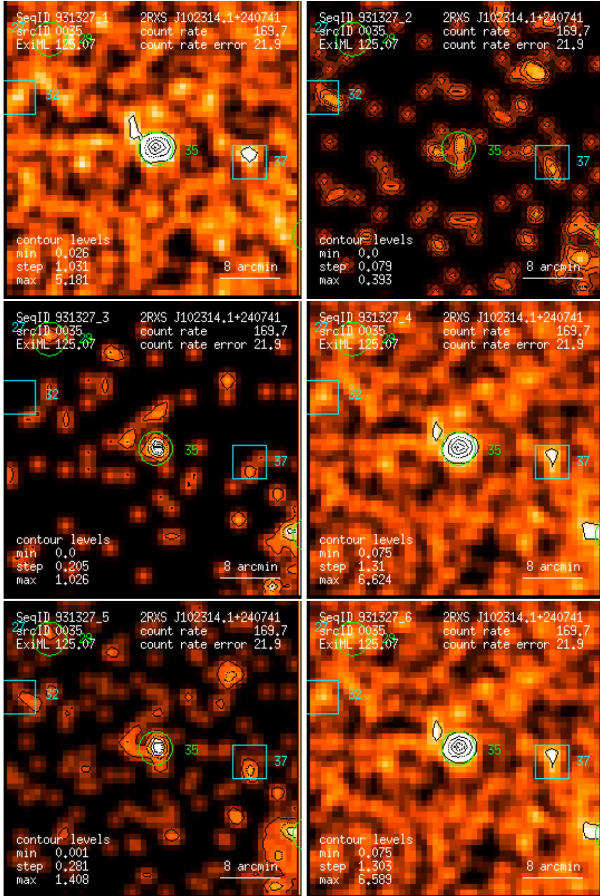
Figure 35: RASS 931327: detection 0035: band rate images, Gaussian filter: (1) PSPC channels 11 – 41, (2) 52 – 90, (3) 91 – 201, (4) 11 – 235, (5) 52 – 201, (6) 11 – 201. Broad band rates in counts/ks. Band rate contour levels in counts/ks/arcmin 2 .
