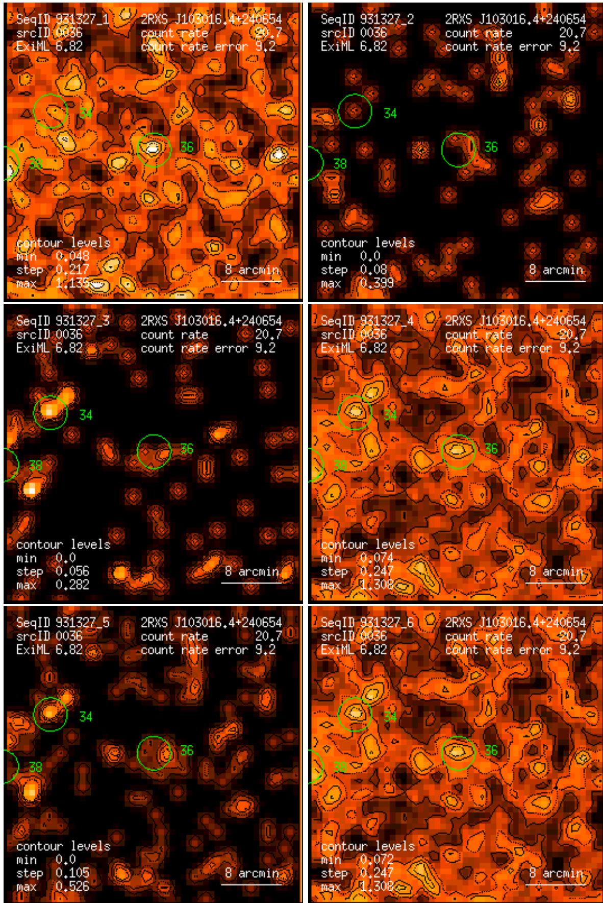
Figure 36: RASS 931327: detection 0036: band rate images, Gaussian filter: (1) PSPC channels 11 – 41, (2) 52 – 90, (3) 91 – 201, (4) 11 – 235, (5) 52 – 201, (6) 11 – 201. Broad band rates in counts/ks. Band rate contour levels in counts/ks/arcmin 2 .
