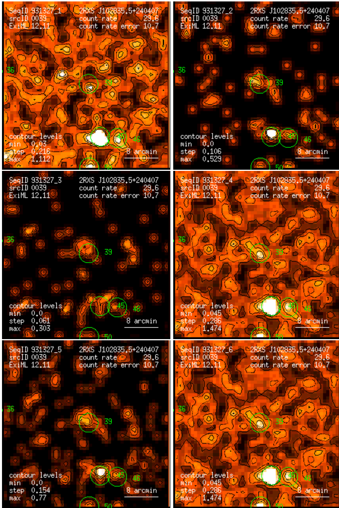
Figure 39: RASS 931327: detection 0039: band rate images, Gaussian filter: (1) PSPC channels 11 – 41, (2) 52 – 90, (3) 91 – 201, (4) 11 – 235, (5) 52 – 201, (6) 11 – 201. Broad band rates in counts/ks. Band rate contour levels in counts/ks/arcmin 2 .
