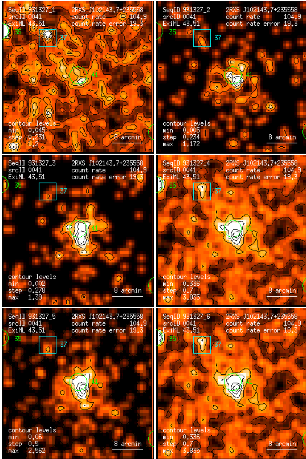
Figure 41: RASS 931327: detection 0041: band rate images, Gaussian filter: (1) PSPC channels 11 – 41, (2) 52 – 90, (3) 91 – 201, (4) 11 – 235, (5) 52 – 201, (6) 11 – 201. Broad band rates in counts/ks. Band rate contour levels in counts/ks/arcmin 2 .
