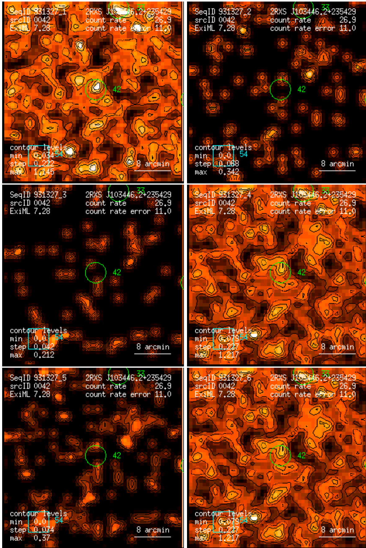
Figure 42: RASS 931327: detection 0042: band rate images, Gaussian filter: (1) PSPC channels 11 – 41, (2) 52 – 90, (3) 91 – 201, (4) 11 – 235, (5) 52 – 201, (6) 11 – 201. Broad band rates in counts/ks. Band rate contour levels in counts/ks/arcmin 2 .
