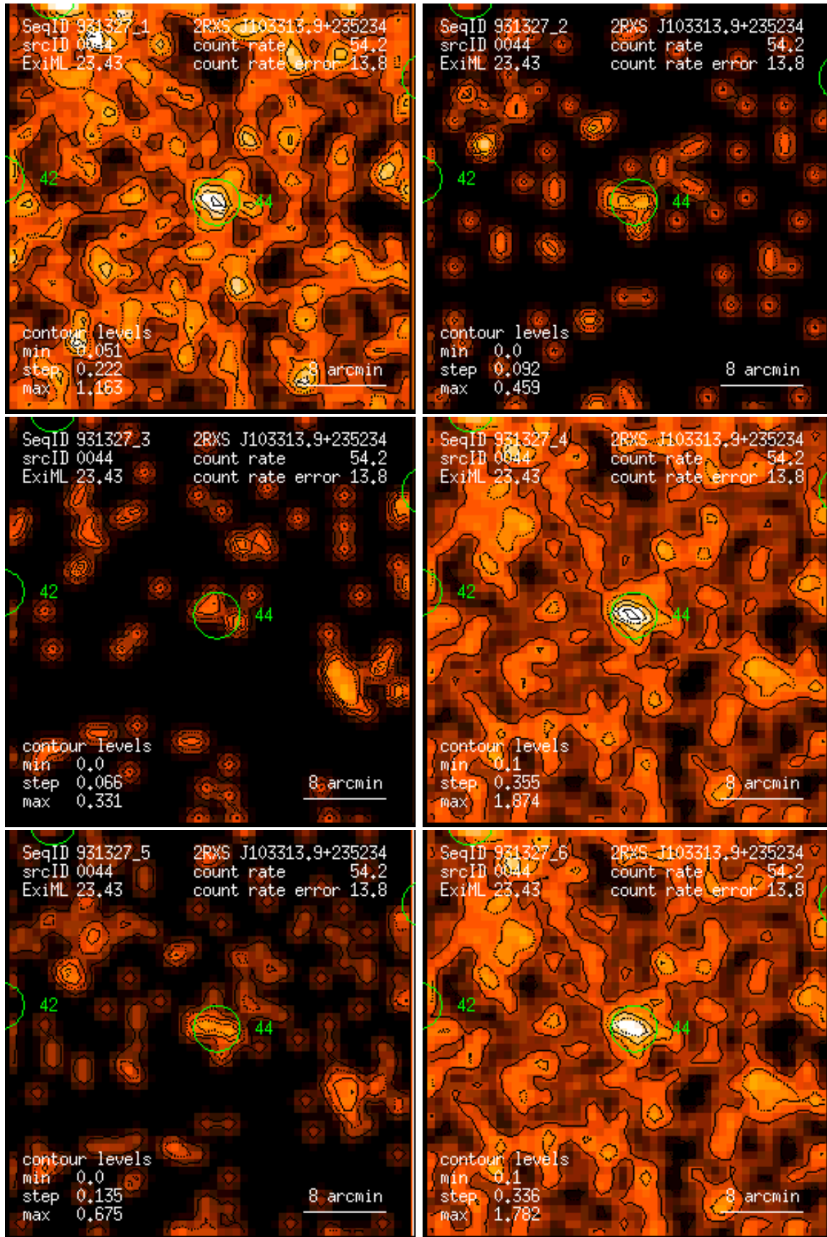
Figure 44: RASS 931327: detection 0044: band rate images, Gaussian filter: (1) PSPC channels 11 – 41, (2) 52 – 90, (3) 91 – 201, (4) 11 – 235, (5) 52 – 201, (6) 11 – 201. Broad band rates in counts/ks. Band rate contour levels in counts/ks/arcmin 2 .
