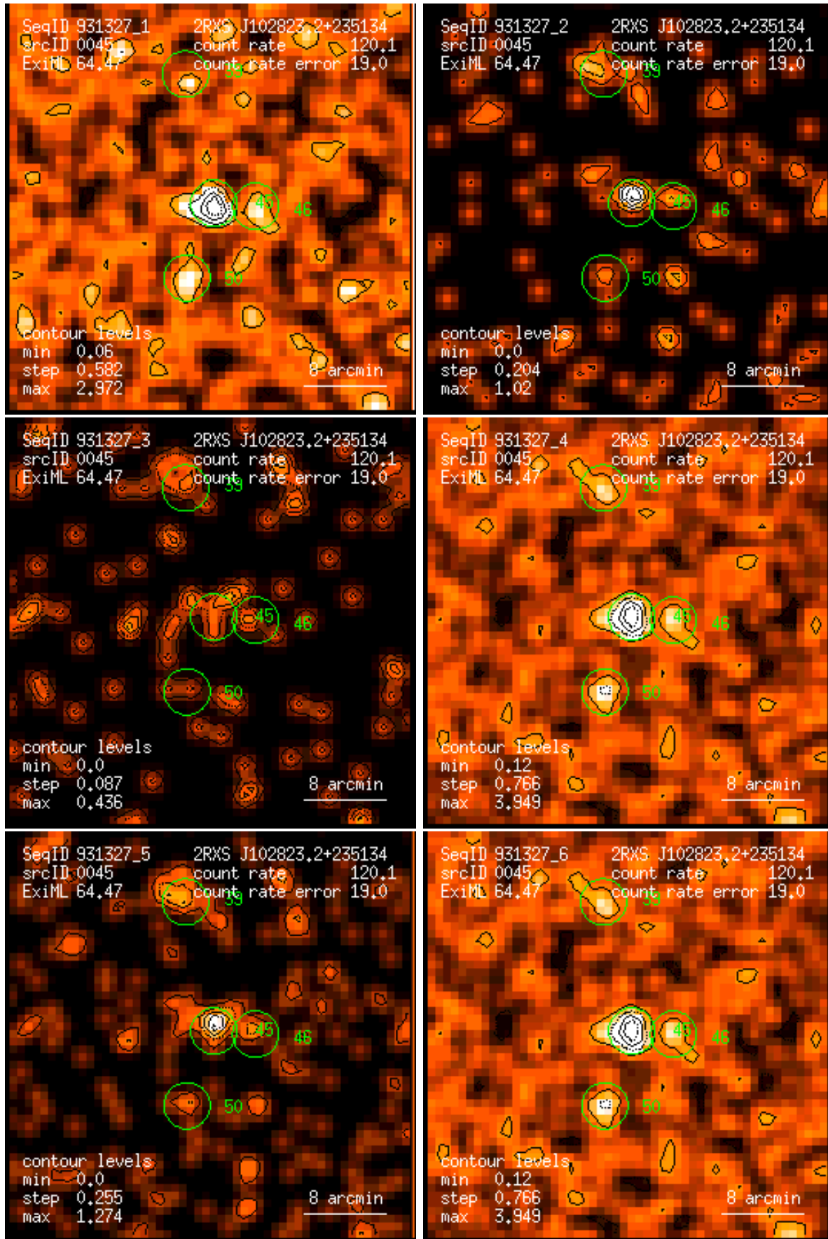
Figure 45: RASS 931327: detection 0045: band rate images, Gaussian filter: (1) PSPC channels 11 – 41, (2) 52 – 90, (3) 91 – 201, (4) 11 – 235, (5) 52 – 201, (6) 11 – 201. Broad band rates in counts/ks. Band rate contour levels in counts/ks/arcmin 2 .
