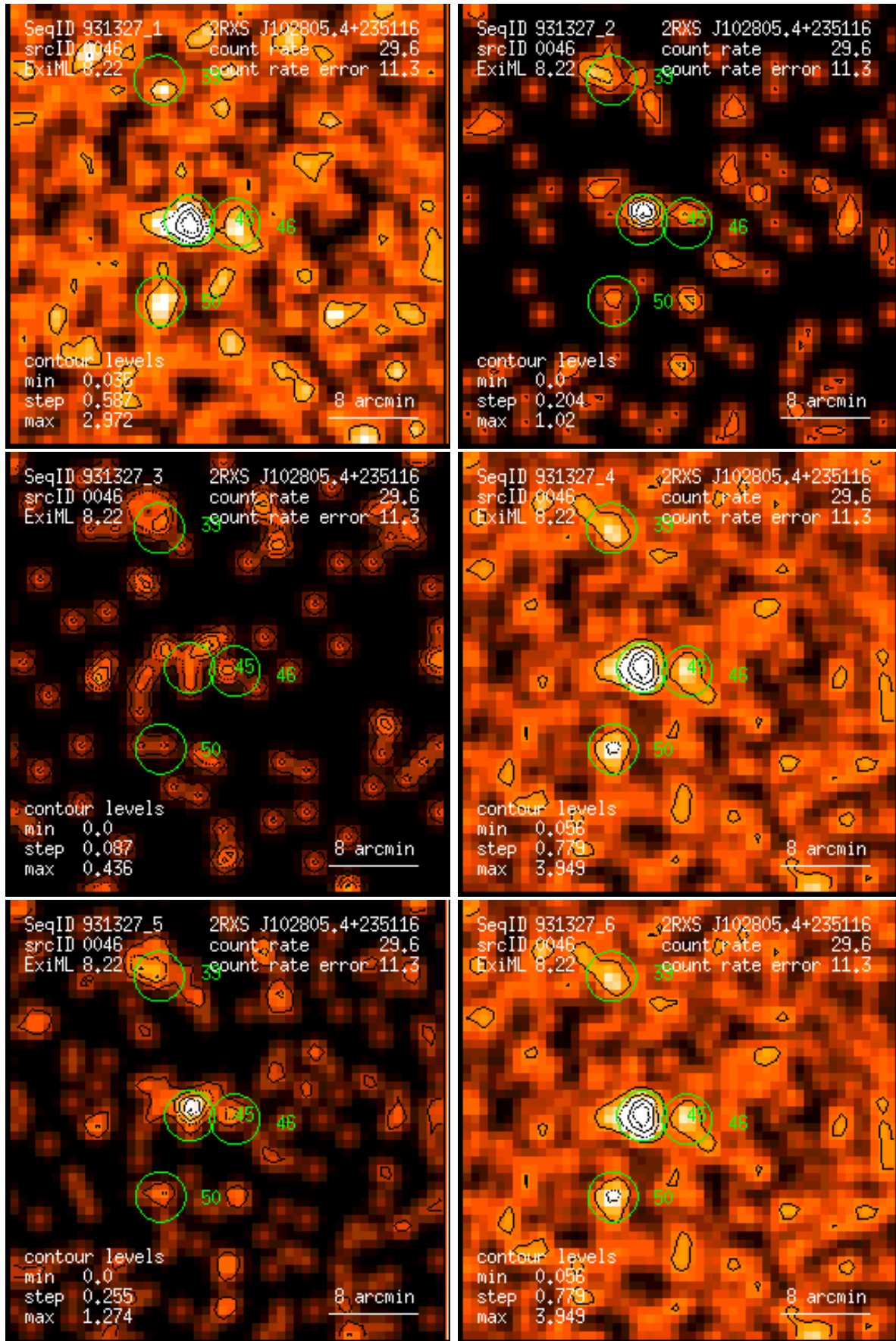
Figure 46: RASS 931327: detection 0046: band rate images, Gaussian filter: (1) PSPC channels 11 – 41, (2) 52 – 90, (3) 91 – 201, (4) 11 – 235, (5) 52 – 201, (6) 11 – 201. Broad band rates in counts/ks. Band rate contour levels in counts/ks/arcmin 2 .
