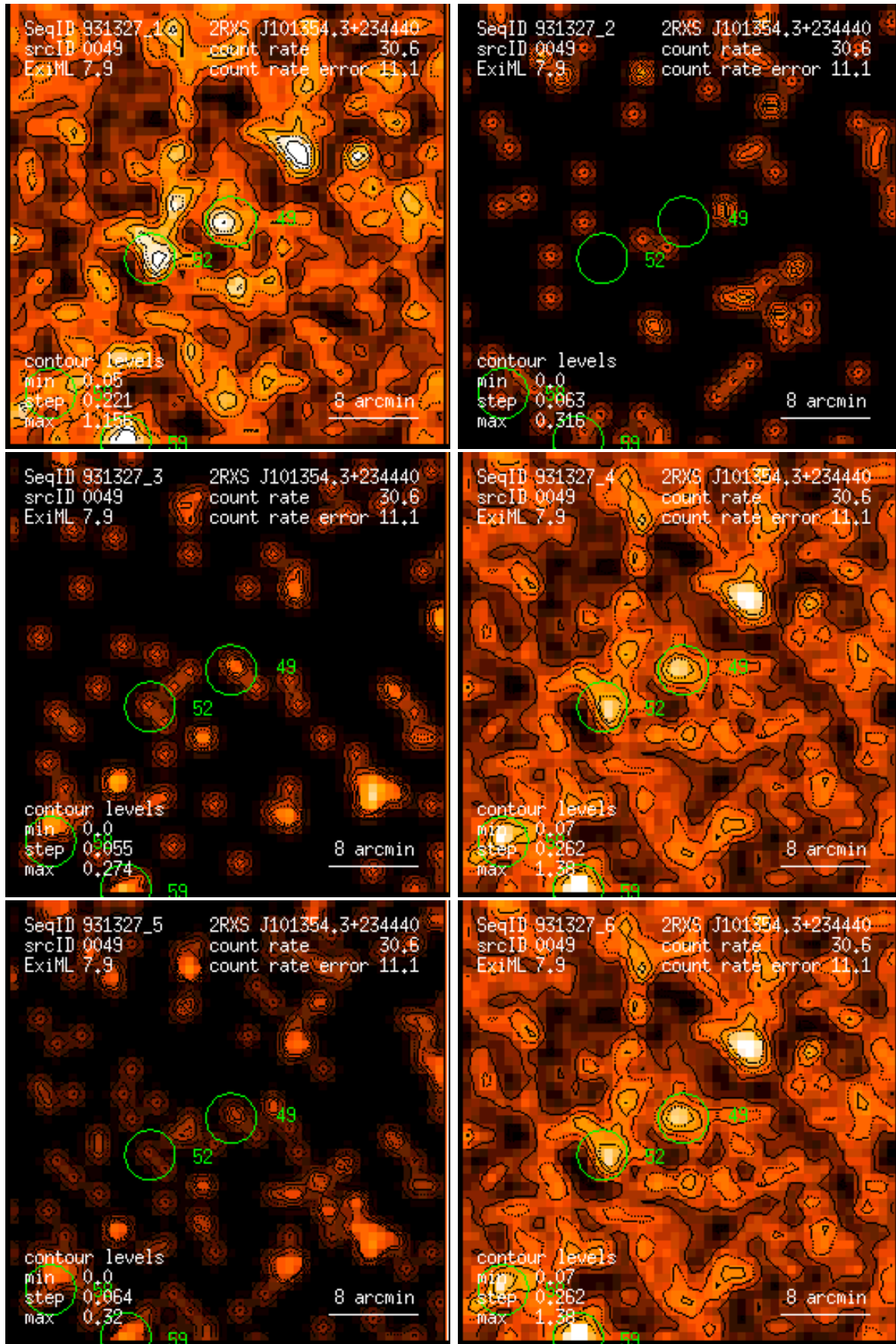
Figure 49: RASS 931327: detection 0049: band rate images, Gaussian filter: (1) PSPC channels 11 – 41, (2) 52 – 90, (3) 91 – 201, (4) 11 – 235, (5) 52 – 201, (6) 11 – 201. Broad band rates in counts/ks. Band rate contour levels in counts/ks/arcmin 2 .
