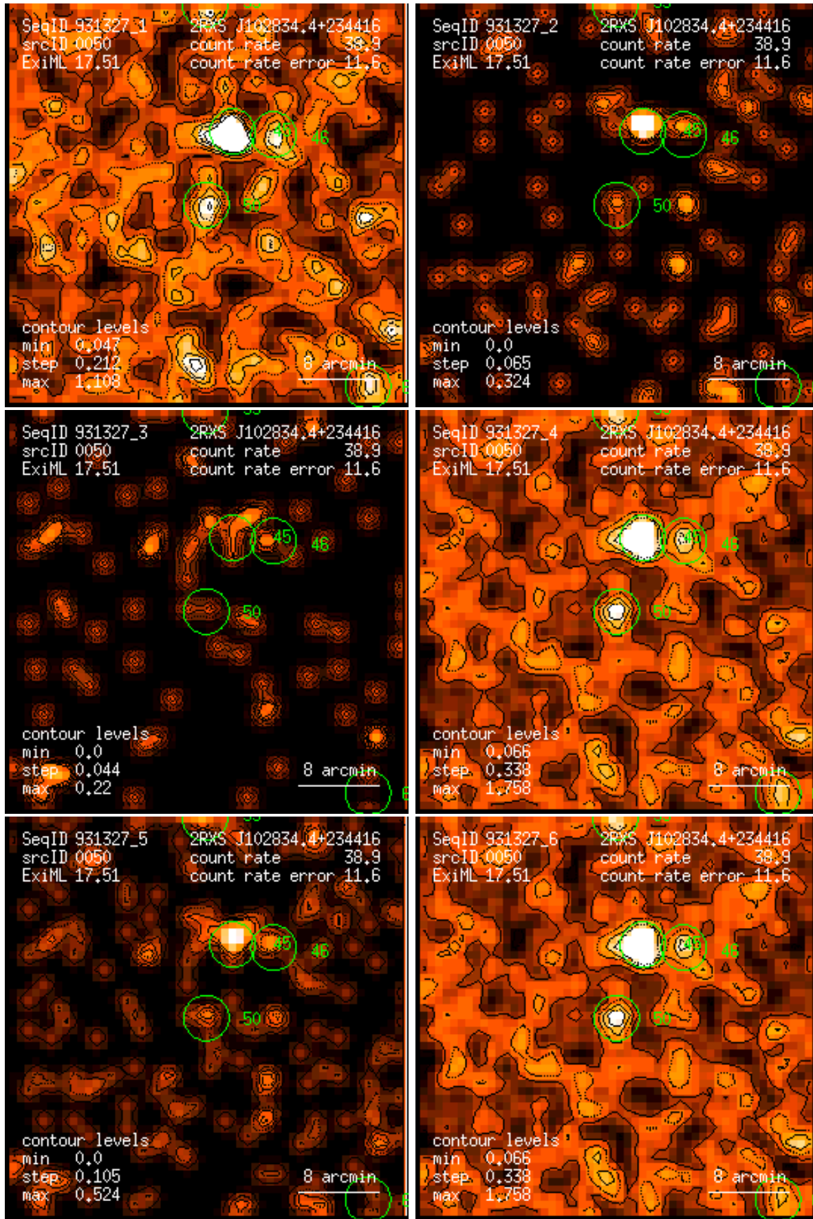
Figure 50: RASS 931327: detection 0050: band rate images, Gaussian filter: (1) PSPC channels 11 – 41, (2) 52 – 90, (3) 91 – 201, (4) 11 – 235, (5) 52 – 201, (6) 11 – 201. Broad band rates in counts/ks. Band rate contour levels in counts/ks/arcmin 2 .
